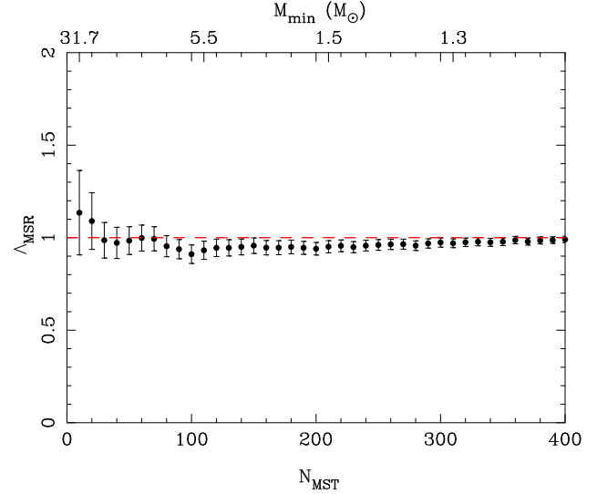
Figure 2. Mass segregation ratio, \Lambda_{\text{MSR}} , for the N_{\text{MST}} most massive stars in the centre of Cyg OB2 in steps of 10 stars using the ‘mass function complete’ sample with 1\sigma error bars. The lowest mass star in each bin is indicated along the top. \Lambda_{\text{MSR}} = 1 , indicating no mass segregation, is shown as a dashed red line.
