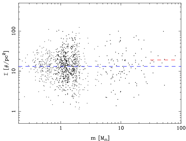
Figure 3. The m - \Sigma distribution for all stars in our dataset showing the local surface density for each star plotted against its mass. Our ‘mass function complete’ sample is shown with black dots, while stars excluded from this sample are shown as grey dots. The median surface densities of all the stars in the ‘mass function complete’ sample (blue dashed line) and that of the 10 most massive stars in the sample (red dashed line) are also shown.
