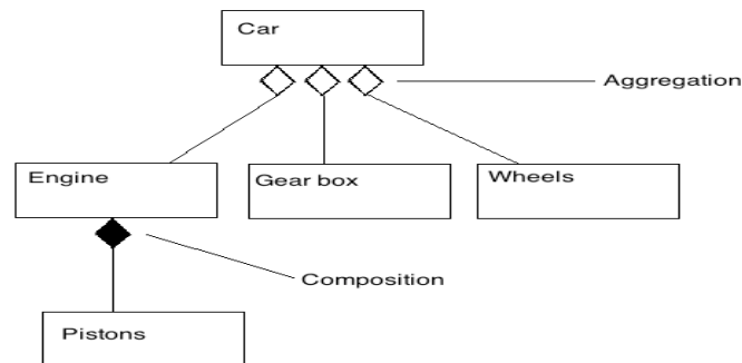
Figure 2 UML notation for Aggregation and Composition.
