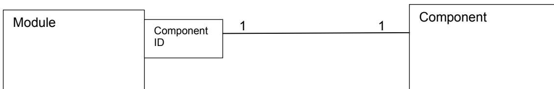
Figure 6 Weak Entity as a qualified association.
