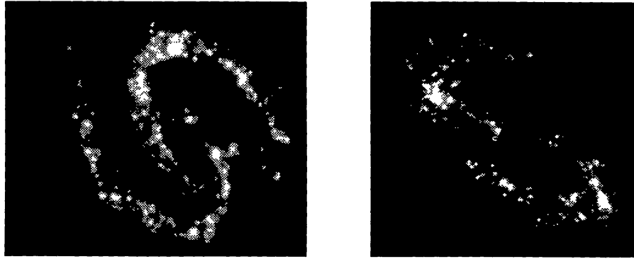
Figure 1. Arm-only images of NGC 157 (left) and NGC 6764 (right). The arm shape has been defined comparing the continuum and H\alpha images of the galaxies.
