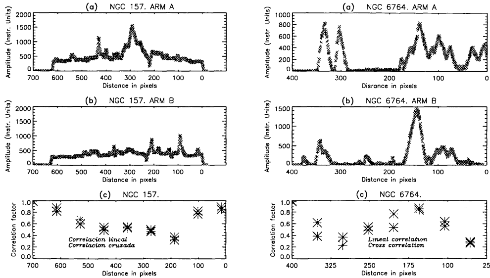
Figure 2. H\alpha luminosity profiles along the two main arms of NGC 6764 and NGC 157, showing H\alpha flux (instr. units) as a function of distance along the arms (pixels). The panels (c) show the values of the linear correlation between these two luminosity profiles (dotted asterisks), and the cross-correlation between the two images of the arms (solid asterisks) for distinct positions along the arms. Note that the centers of the galaxies are plotted on the right-hand sides.
