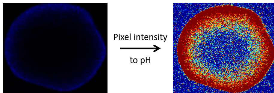
Figure 1: Conversion of pixel intensity to pH. Image on left is produced by the division of the pixel intensities of a picture showing pHrodo fluorescence by the corresponding FITC image. Image on right is the result of coloration of the left image based on the intensity of each pixel.
