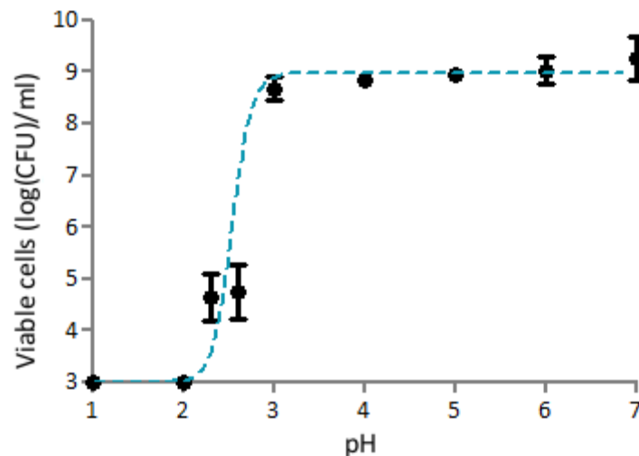
Figure 2: Viability of B. breve against TPY medium adjusted to various pH after 1 hour incubation at 37°C. N=3, \pm standard deviation. Limit of detection: 3 log(cfu)/mL. Line intended as guide to eye.
