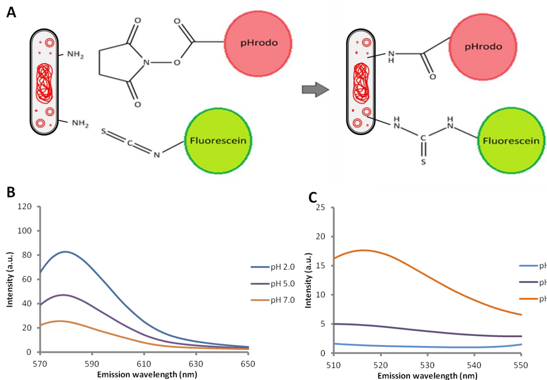
Figure 4. Schematic diagram of dye conjugation to amine moieties within bacteria, producing thiourea and amide moieties when reacting with pHrodo succinimidyl ester and FITC, respectively (A). Fluorescence of pHrodo (B) and FITC (C) when conjugated to B. breve showing variation of intensity with pH. For this experiment, a solution of fluorescently labelled B. breve conjugate (100 \mu L) at \sim 9 log(cells)/mL was diluted into PBS (900 \mu L)
