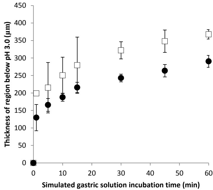
Figure 7: Encroachment of pH < 3.0 into alginate (open squares) and chitosan-coated alginate (closed circles) matrices during incubation in simulated gastric solution at 37 °C. N=3 ± standard deviation, band thickness is the average of 5 measurements at equidistant points on the matrix.
