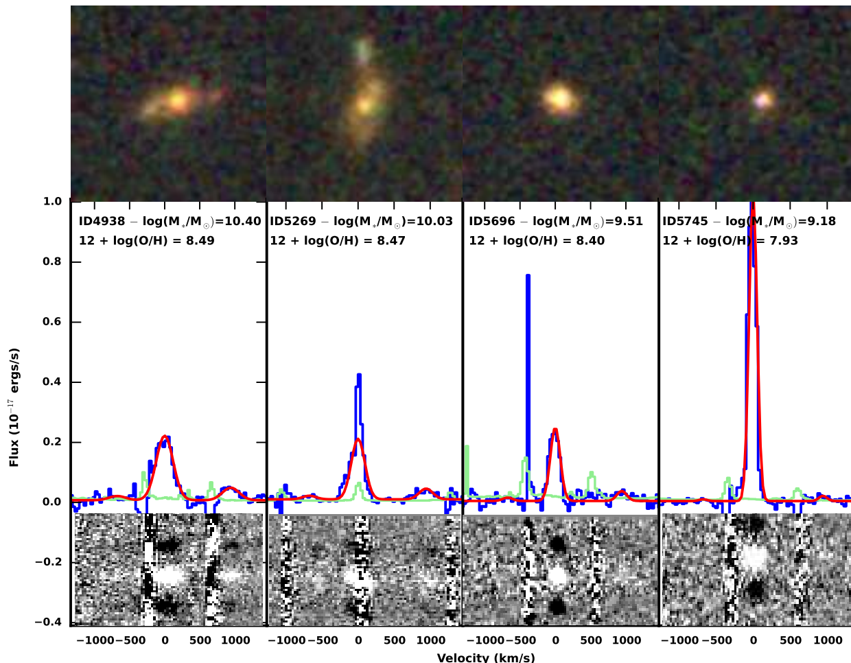
FIG. 1.— Representative sample of flux-calibrated 1D and 2D MOSFIRE spectra of four cluster members in order of decreasing stellar mass. The spectra are plotted with respect to the systemic velocity of each galaxy, as defined by their nebular emission-lines. Both the [N II] doublet and H \alpha are shown in the 1D and 2D spectra. Strong sky-lines are seen as long vertical lines in the 2D spectra. The 1D data (blue), 1\sigma error spectra (green) and best-fit Gaussian models (red) are shown. The metallicity for each object is also listed. The top panels show 4'' \times 4'' three color HST images, using the F814W, F125W and F160W filters, obtained from the publicly available CANDELS data (Grogin et al. 2011; Koekemoer et al. 2011; Skelton et al. 2014).
