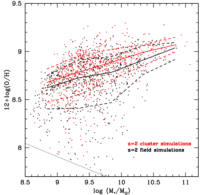
FIG. 3.— Mass-metallicity relation for simulated field (black) and cluster (red) galaxies. The solid and dashed lines show the moving median with 68% of confidence level. The dotted line is an observational limit of our ZFIRE survey (see text for details). We find that both field and cluster galaxies have consistent mass-metallicity relations with maximum separations of 0.1dex.
