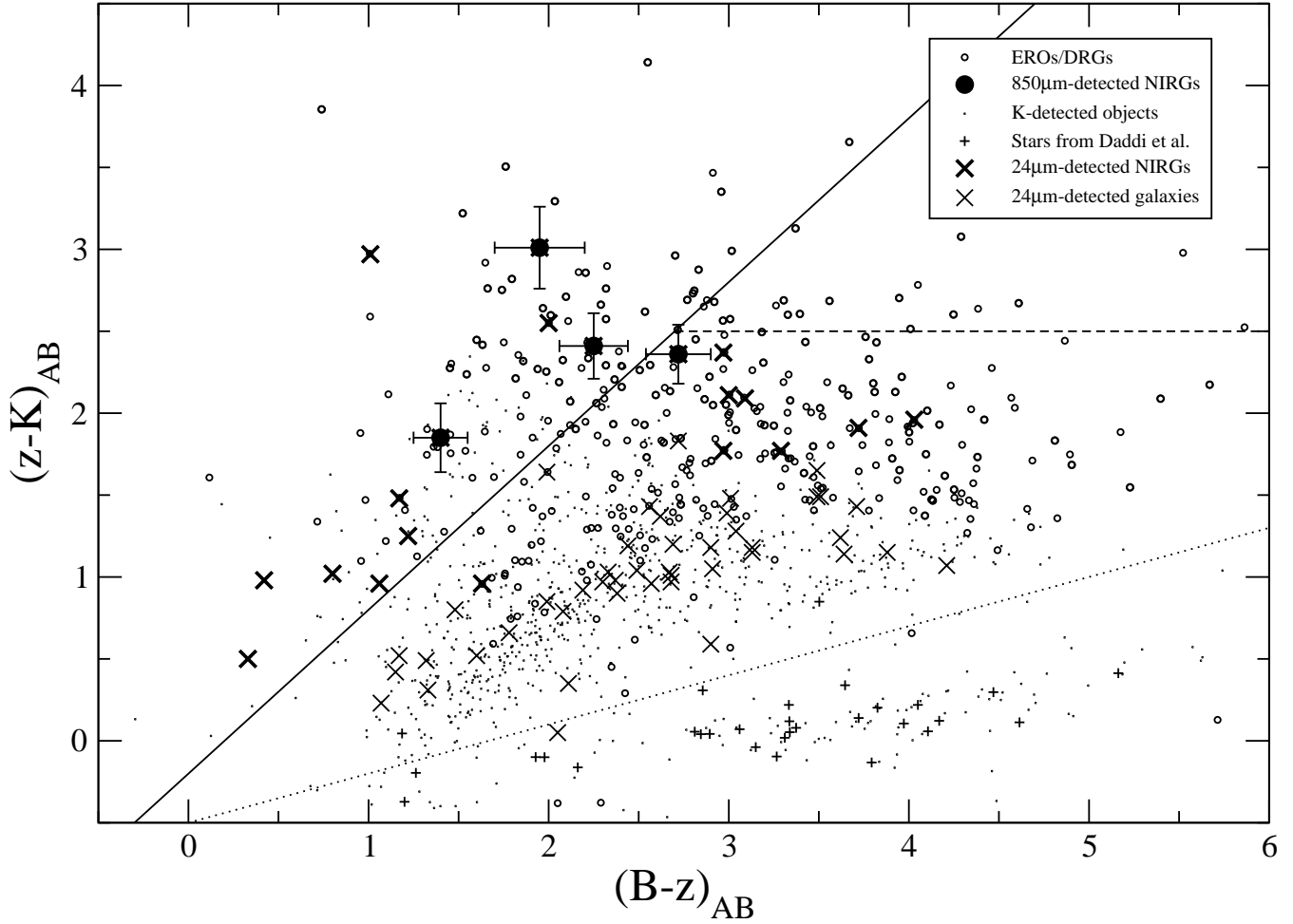
Figure 7. The BzK diagram for K_s -detected sources in the SXDF/SIRIUS field. Solid circles indicate submm-bright NIRGs. The photometric errors include those of colour corrections on B-z and z-K . Both EROs and DRGs are indicated with small circles. Large thick/thin crosses are for NIR-selected/ K_s -detected galaxies which are detected at 24 \mu m with SWIRE. Small pluses indicate stars from Daddi's catalogue. We depict the BzK -selection criterion with a solid line. Dashed and dotted lines are boundaries for selecting passively evolving galaxies and stars, respectively.
