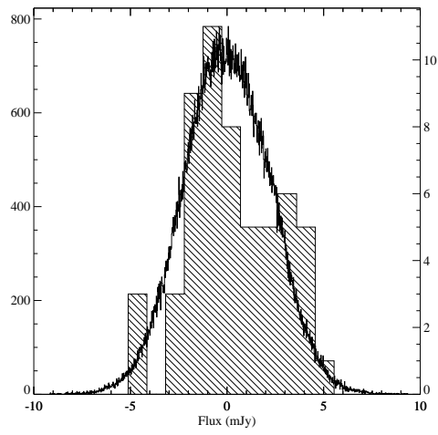
Figure 6. Same as Figure 4, but for DRGs.
