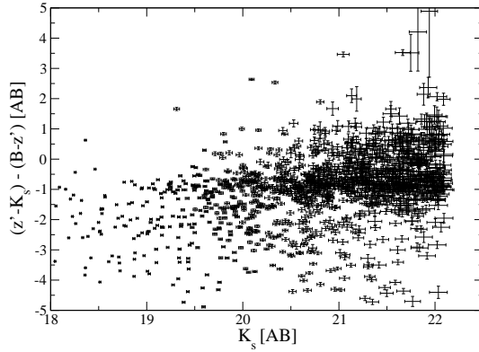
Figure 2. BzK colour vs. K_s magnitude for K_s -band detected objects. Here the z' - K_s and B - z' colours have not been colour-corrected in order to show the original photometric errors. The BzK selection criterion proposed by Daddi et al. (2004) corresponds to (z' - K_s) - (B - z') = 0.2 for the adopted colour correction (see text).
