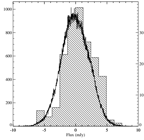
Figure 5. Same as Figure 4, but for EROs.
