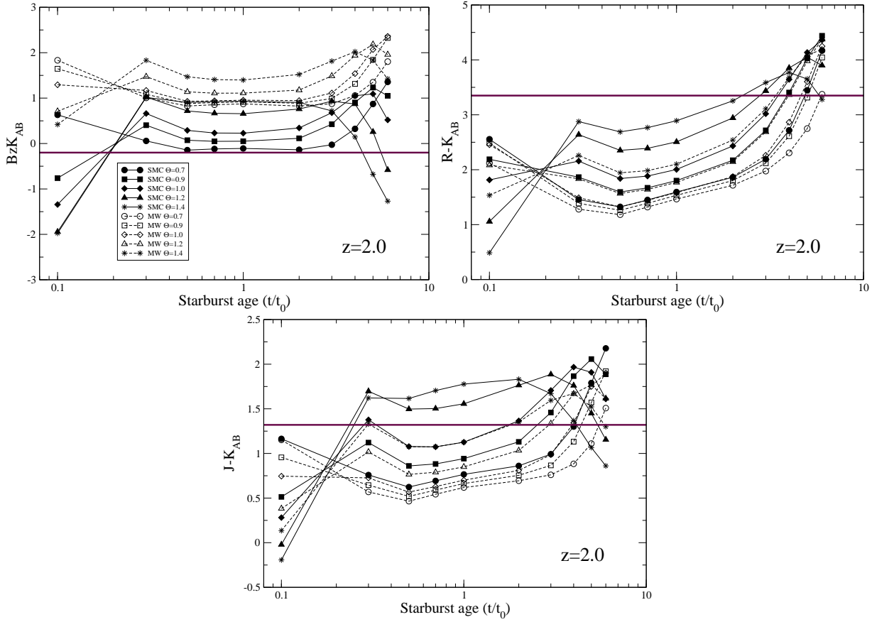
Figure 10. BzK , R-K and J-K colours of the SBURT model at z = 2 as a function of starburst age, which show the range of model parameters to satisfy BzK , DRG, and ERO selection criteria. Model parameters for a given line symbol are shown in the legend box. Horizontal lines indicate the colour boundary for BzK s, DRGs and EROs.
