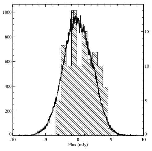
Figure 4. Histograms of the 850- \mu m flux at the position of BzKs (shaded; right axis), compared to the histograms for the unmasked regions of the SCUBA map as a whole (open; left axis).
