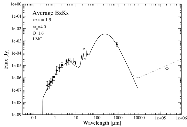
Figure 11. Average SED of BzK s with 1.5 < (B - z') < 2.5 and a representative SBURT model for the average SED. Symbols are the same as in Figure 8.
