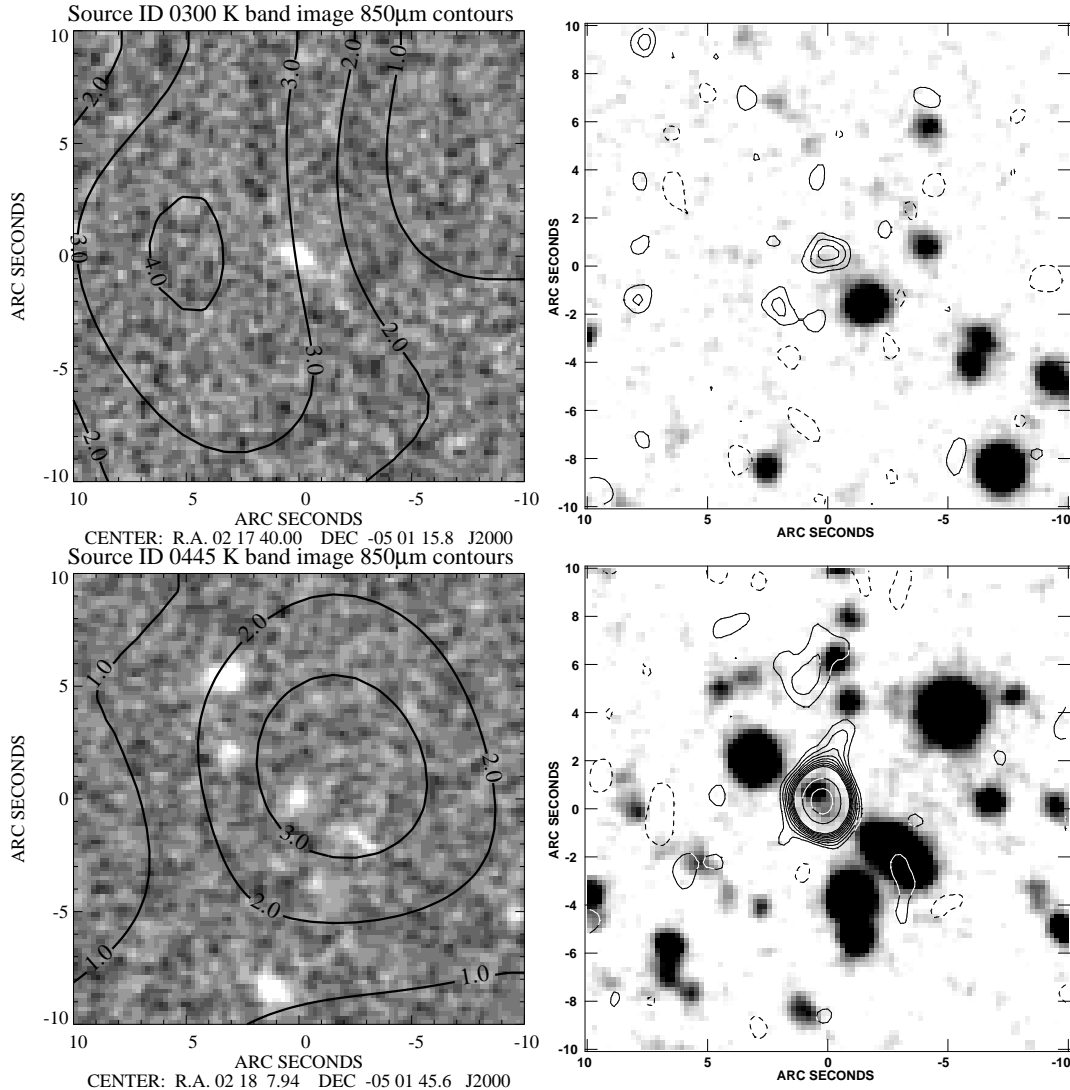
Figure 3. [Left column] Contours of SCUBA 850\text{-}\mu\text{m} for submm-bright NIR-selected galaxies. The corresponding S/N ratios at 850\text{ }\mu\text{m} are indicated at each contour line. The underlying images are K_s -band with 20'' on a side. The names of the sources are indicated at the top of each image. [Right column] Contour maps of radio (1.4 GHz) on negative images at R -band for the same regions as shown in the left panels. Contour lines are shown at -2, 2, 3, 4, \dots, 10, 20, \dots, 100 \times \sigma . Positive (negative) contours are indicated with solid (dashed) lines.
