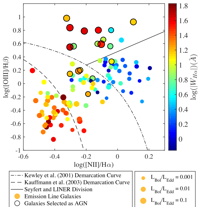
Figure 2. BPT diagram for the Pimblet et al. (2013) galaxies with \text{SNR} > 3 in each of the four emission lines and with mass greater than 10^{10.4} M_{\odot} . Point colours represent H\alpha equivalent widths and sizes represent \log(L_{\text{Bol}}/L_{\text{Edd}}) , with the largest points corresponding to the largest L_{\text{Bol}}/L_{\text{Edd}} values. AGN (black circles) are those galaxies which satisfy: |W_{H\alpha}| > 3 \text{ \AA} (yellow-green points), L_{\text{Bol}}/L_{\text{Edd}} > 0.01 (large points), lie above the Kauffmann et al. (2003) demarcation curve (dashed curve) and are closer to the Kewley et al. (2001) demarcation curve (dot-dashed curve) than to the Kauffmann et al. (2003) curve.
