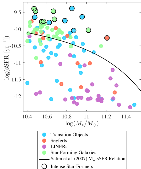
Figure 3. sSFR against stellar mass for the Pimblet et al. (2013) galaxies with \text{SNR} > 3 in each of the four emission lines and with mass greater than 10^{10.4} M_{\odot} . Point colours show the BPT classification of each galaxy. Intense star-formers (black circles) have sSFRs above the expected sSFR (black curve) by > 1.5\sigma .
