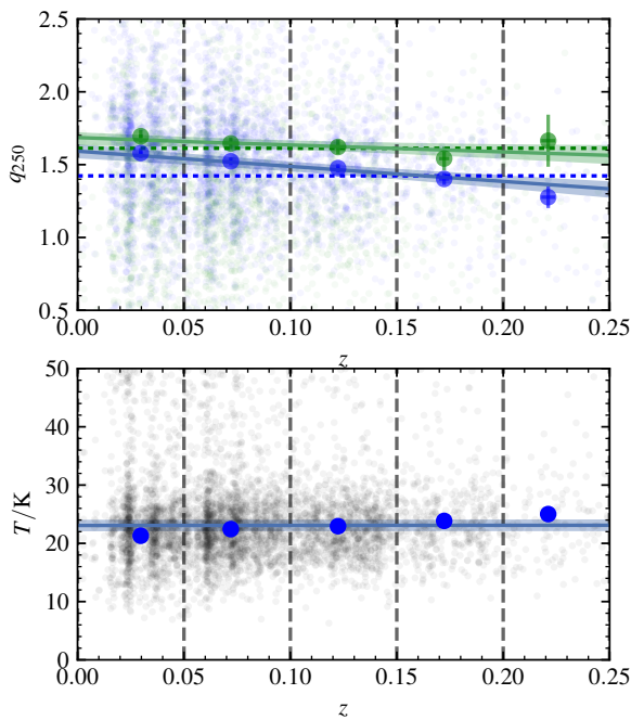
Figure 8. Top: Evolution of q_{250} over redshift measured with LOFAR at 150MHz (blue) and FIRST transformed to 150MHz (green). The dashed horizontal line in the upper plot is the mean-stacked q_{250} for all star-forming galaxies taken from Figure 6 for FIRST and LOFAR at 150MHz. The coloured lines indicate the straight line fit to all galaxies in our sample binned in redshift for LOFAR and FIRST. Bottom: The temperature in each bin, calculated by constructing an infrared SED from the average K -corrected flux of each source in every band and fitting Equation 2 to the result. The temperature and uncertainties are overlaid with a straight line fit to the data. The vertical dashed lines represent bin edges.
