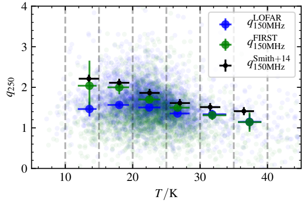
Figure 9. The temperature dependence of q_{250} compared between high and low frequency. The background dots are the individual q_{250} calculated from the LOFAR 150MHz (blue) and FIRST (green) luminosity densities. The q_{250} calculated from stacked LOFAR and SPIRE luminosity densities described earlier is plotted in bold points with errorbars derived from bootstrapping the luminosity densities within the depicted dashed bins 10,000 times. The temperature uncertainties in each bin are calculated from the 16th and 84th percentiles. The same calculation from Smith et al. (2014) is shown as the black errorbars for comparison.
