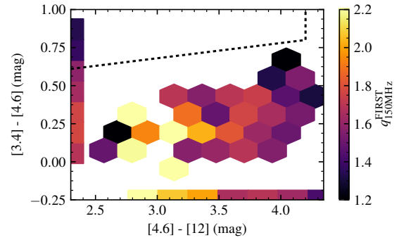
(b) FIRST transformed to 150MHz assuming \alpha = -0.71
