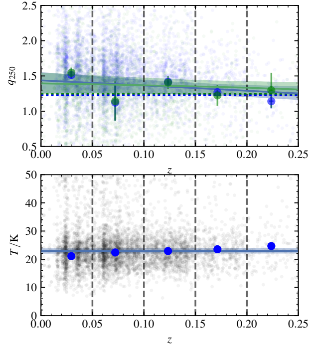
Figure A1. Top: Evolution of q_{250} over redshift measured with LOFAR at 150MHz (blue) and FIRST transformed to 150MHz (green). This plot uses our star-forming sample merged with BPT-AGN whose emission lines are detected at 5\sigma . The dashed horizontal line in the upper plot is the mean-stacked q_{250} taken from Figure 6 for FIRST and LOFAR at 150MHz. The coloured lines indicate the straight line fit to all galaxies in our sample binned in redshift for LOFAR and FIRST. Bottom: The temperature in each bin, calculated by constructing an infrared SED from the average K -corrected flux of each source in every band and fitting Equation 2 to the result. The temperature and uncertainties are overlaid with a straight line fit to the data. The vertical dashed lines represent bin edges.
