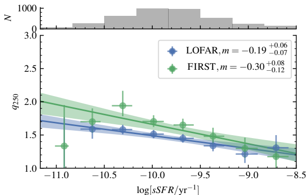
Figure 13. q_{250} for LOFAR (blue) and FIRST (green) at 150MHz against the specific star formation rate in 7 bins of width 0.3 dex. The uncertainties on q_{250} are calculated via bootstrapping within each bin. The uncertainties on sSFR are calculated from the 16th and 84th percentiles in each bin. Straight line fits are shown as coloured lines with 1\sigma credible intervals shown as shaded regions. The top histogram shows the number of galaxies in each bin.
