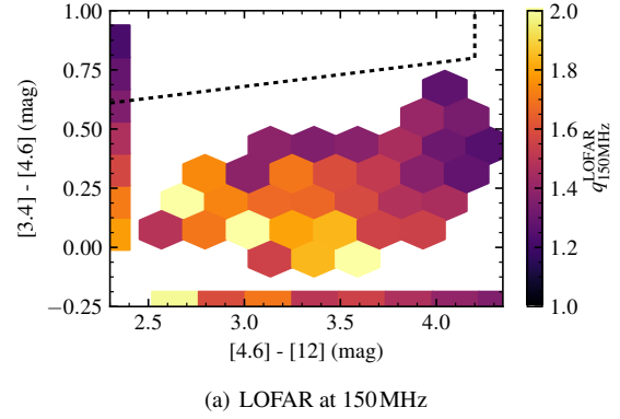
(a) LOFAR at 150MHz
