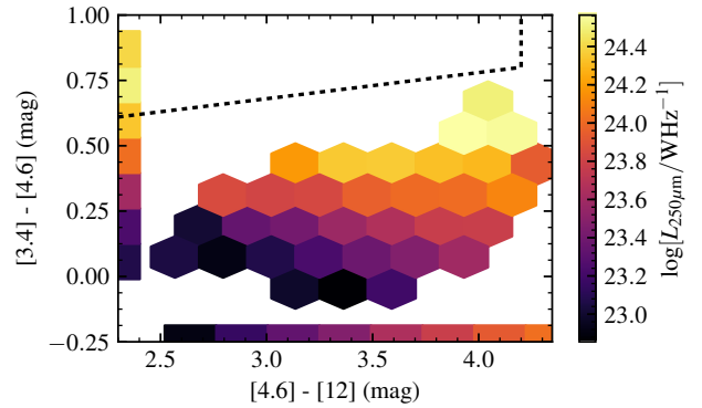
(c) 250 \mu m
