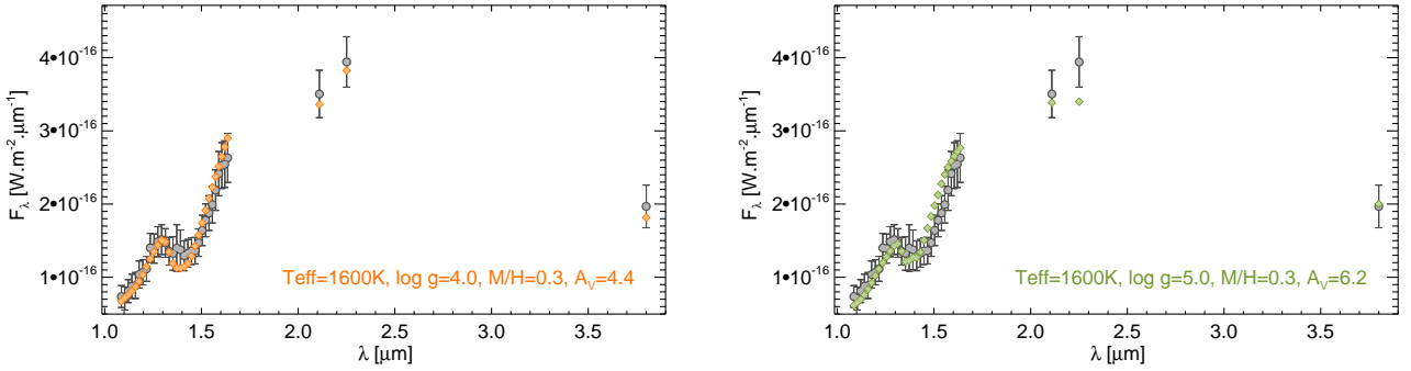
Fig. 19: Left: Best fit of observation (in black) with reddened BT-Settl atmosphere (in orange). Right: Best fit ( \chi^2 ) with reddened BT-Settl atmosphere when forcing higher gravity.
