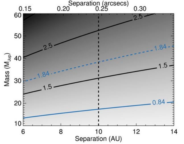
Fig. E.1: Mass limit for the observed \Delta\mu adopting R_0 = 1 in the Makarov & Kaplan (2005) equation. (corresponding to pole-on circular orbit) The solid blue line represents the observed \Delta\mu value, the dashed line the 1\sigma limit.
