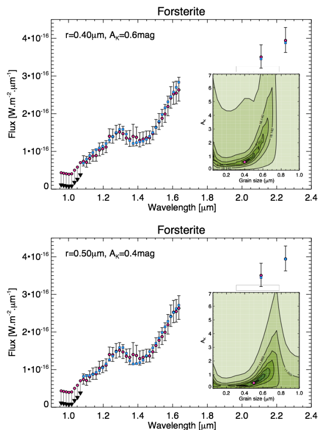
Fig. 11: Comparison of the spectrum and photometry of HD 206893b (pink dots) to that of the L7 red dwarf PSO_J057.2893+15.2433 (bottom, Liu et al. 2013) and the L0 optical standard dwarf 2MASS J0345432+254023 (top, Kirkpatrick et al. 1997) reddened by a layer of forsterite grains with mean sizes of 0.50 and 0.40 \mu\text{m} , respectively. The mean flux of the reddened template spectrum is re-normalised to fit that of the companion. The G map is overlaid in the lower right portion of the plots.
