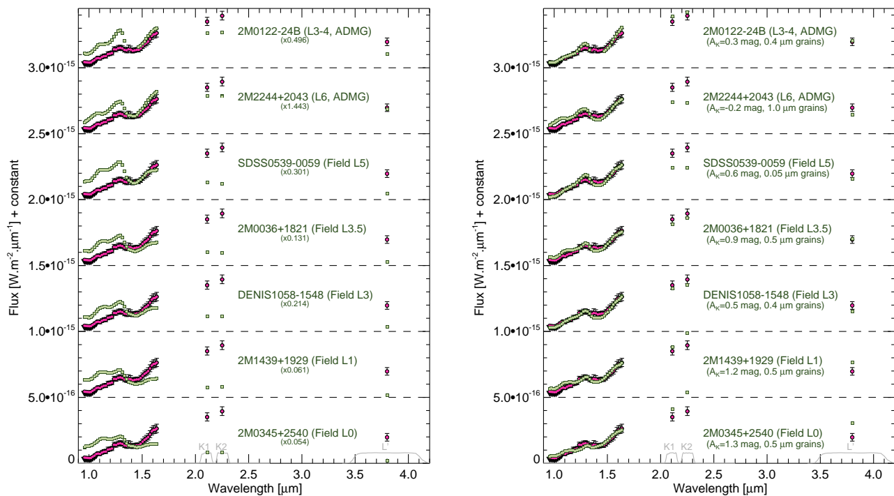
Fig. 13: Comparison of spectral energy distribution of HD 206893b to those of flux-calibrated spectra of benchmark objects re-scaled to the distance of HD 206893b. On the left, the template spectra are re-normalised by an additional factor to match the flux of HD 206893. On the right, they are reddened by forsterite grains, but an additional normalisation factor is not applied.
