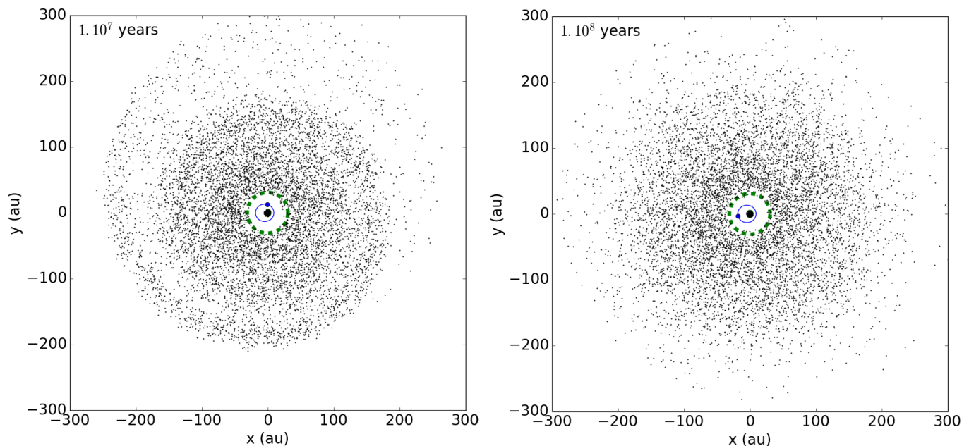
Fig. 22: Representation of an N-body simulation of 10,000 test particles initially ranging from 1 to 200 AU after (a) 10 million years (b) 100 million years. A companion has been injected at t=0 with semi-major axis 14.2 AU and eccentricity 0.31. Its orbit is depicted in blue, while the gap outer extent given by Eq. 4 is in green.
