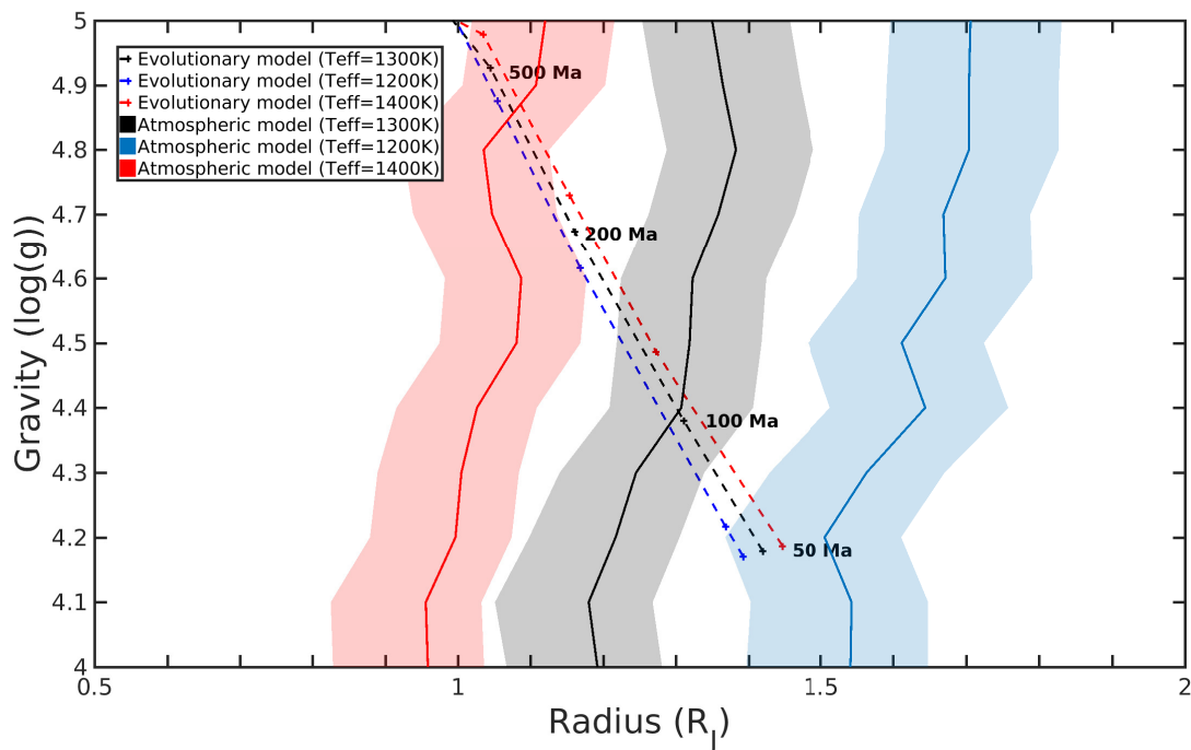
Fig. 14: Radius and gravity associated with atmosphere models (full line) and evolutionary models (dashed line). The shaded area corresponds to the uncertainty on the radius of the atmosphere models to match the absolute flux of HD 206893B. We used the ExoREM atmosphere models, which provide the best fit to HD 206893B (see Sect. 5.3), and the Baraffe et al. (2003) evolutionary models.
