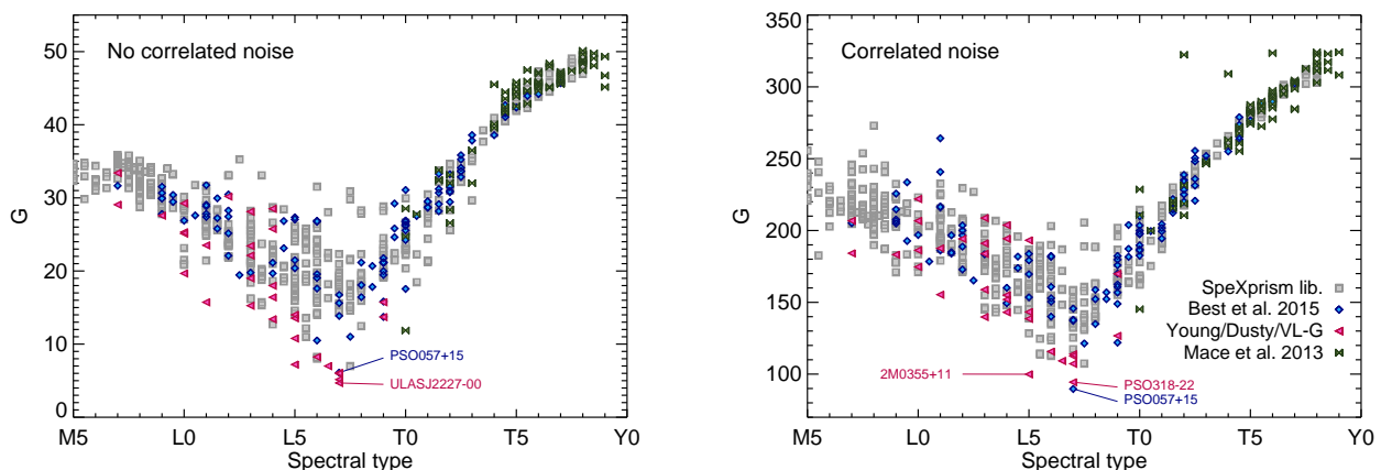
Fig. 8: Comparison of the NIR spectrum and photometry of HD 206893b to those of reference spectra. On the left the fit does not account for the correlation noise of the IFS spectrum; on the right, it does.
