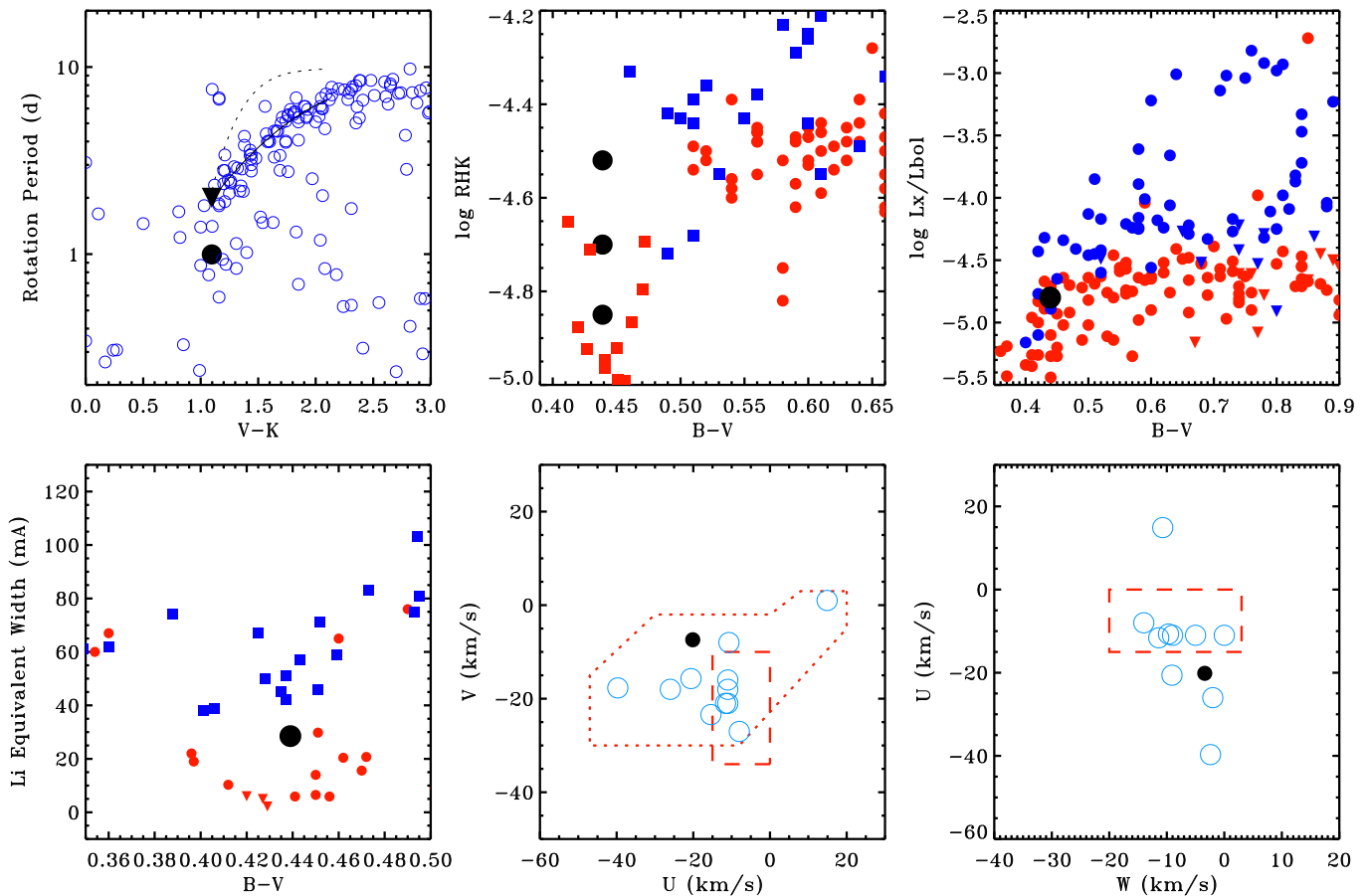
Fig. 1: Comparison of rotation period, chromospheric emission \log R_{HK} , coronal emission \log L_X/L_{bol} , and Li EW of HD 206893 to those of the Hyades (red symbols) and Pleiades (blue symbols) open clusters. In the first panel (rotation period), the filled circle shows the photometric period and the triangle the upper limit derived from the projected rotational velocity. In the same panel the continuous and dashed lines are the sequences of slow rotators for Pleiades and Praesepe, respectively (Stauffer et al. 2016). They overlap at the colour of HD 206893. The last two panels show the kinematic parameters of HD 206893 and those of several young moving groups. In these panels, the dashed box represent the locus of the Nearby Young Population as defined in Zuckerman et al. (2004). The dotted contours in the U vs V plot mark the locus of kinematically young stars, as proposed by Montes et al. (2001).
