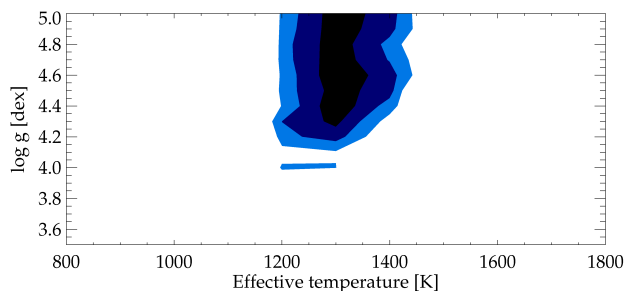
Fig. 17: \chi^2 contour map of ExoRem atmosphere model fits at solar metallicity. Deep blue is the 1\sigma contour, blue is 2\sigma , and light blue is 3\sigma .
