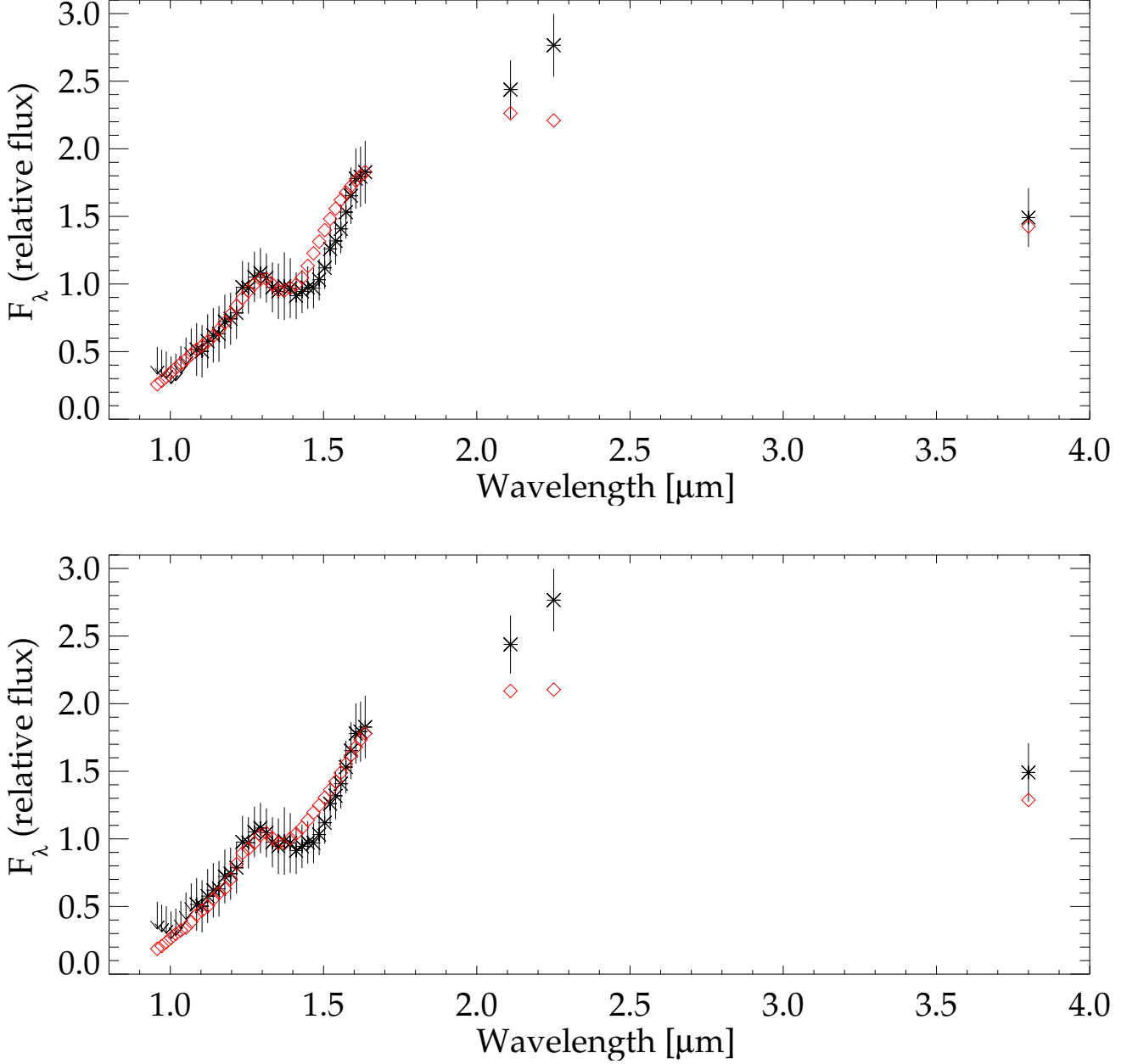
Fig. 16: Upper panel: Best fit Exorem atmosphere model (1300 K, [M/H]=0.0 , \log g =4.4 , in red), compared to the HD 206893B spectrum (in black). Lower panel: Best fit Exorem atmosphere model when super-solar metallicity is forced (1500 K, [M/H]=0.5 , \log g =4.5 , in red), compared to the HD 206893B spectrum (in black).
