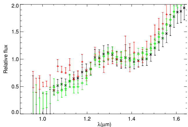
Fig. B.1: Extracted spectrum of HD 206893B through TLOCI-ADI (black), VIP Optimal-PCA (red), and ANDROMEDA (green)
