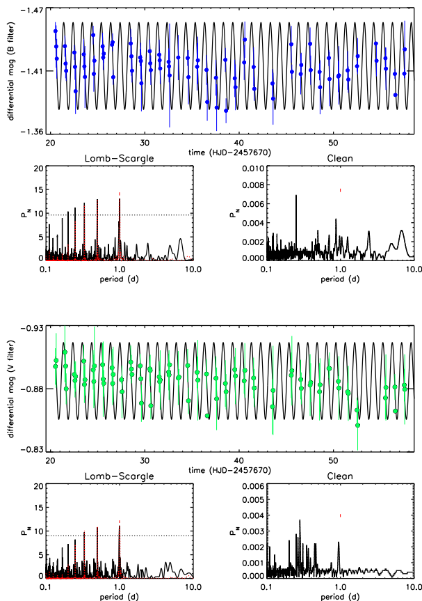
Fig. 2: Results of photometric analysis of HD 206893 for B (top) and V filter (bottom) data. We plot the differential magnitude time series, the Lomb-Scargle periodogram (red line is the window function, dotted line the power at 99% confidence level), the Clean periodogram, and the light curve with the sinusoid fit overplotted.
