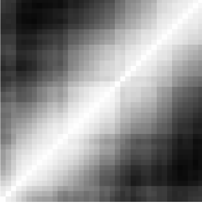
Fig. C.1: Correlation matrix of the noise in the residual image TLOCI-ADI analysis. The x- and y-axes have 39 values associated with the 39 IFS channel. The pixel i, j therefore identifies the correlation of noise between channels i and j . We use a linear scale for which a perfect correlation of 1 is white and a slight anticorrelation of -0.1 is black.
