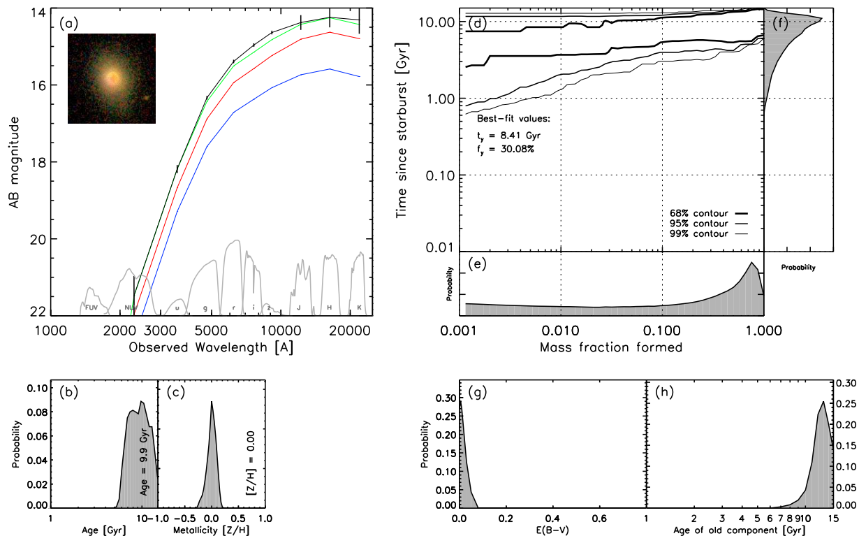
Figure 6. An example of a galaxy where we cannot quantify the first significant episode of star formation, but can place strong limits on the recent star formation history. For a detailed description, see section 3.5.
