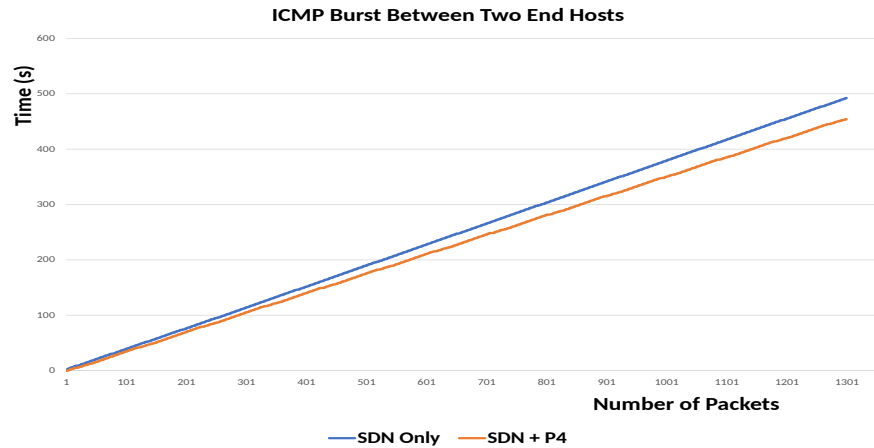
Fig. 8. Illustration of the ICMP Bursts in the Two Environments for 1300 Packets
