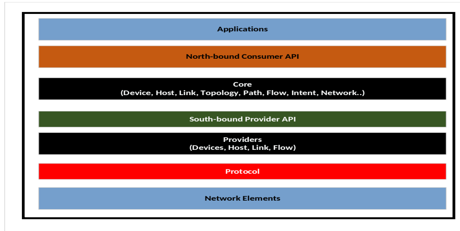
Fig. 1. The illustration represents the ONOS with differentiated tiers of functionalities as presented at [13]
