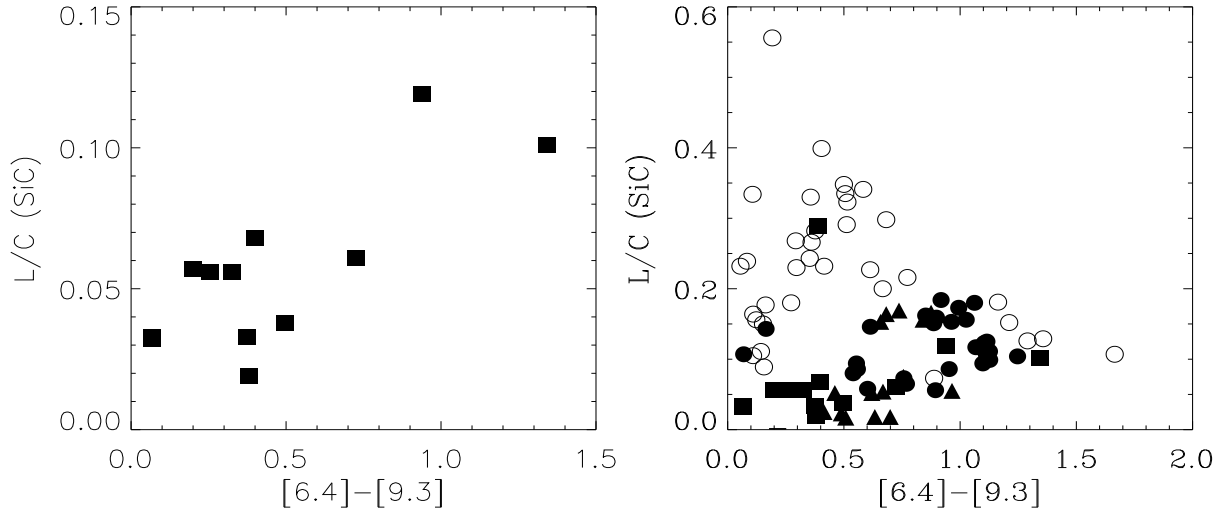
Figure 12. The strength of the SiC feature as a function of the [6.4]–[9.3] colour in our SMC sample (left panel). The right panel combines this with stars from Sloan et al. SMC and Galactic samples: filled squares represent our SMC sample, triangles Sloan et al. (SMC), open circles Sloan et al. (Galactic) sample and filled circles Zijlstra et al. (LMC).
