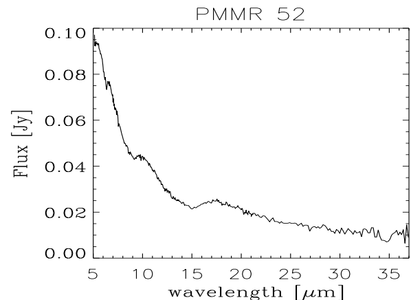
Figure 5. Spectrum of the oxygen-rich star PMMR 52. Typical spectral features of silicates are observed at 9.8 \mu m and 18 \mu m.
