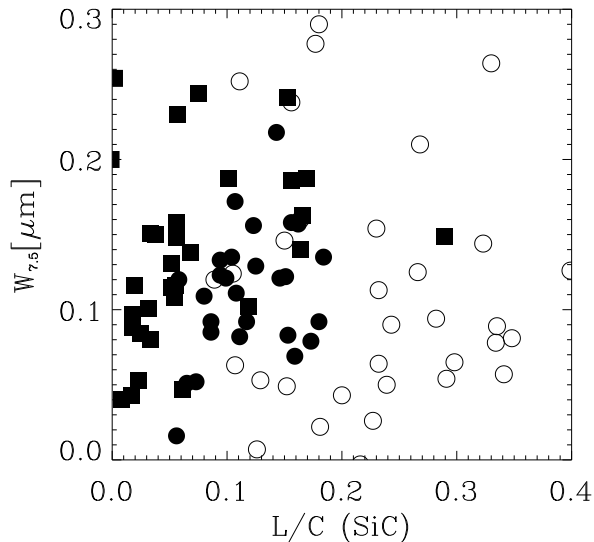
Figure 17. The strength of the C_2H_2 7.5\mu m feature as a function of the SiC feature. Squares represent SMC stars from our sample and Sloan et al. sample, black circles Zijlstra et al. LMC sample and open circles Sloan et al. Galactic sample.
