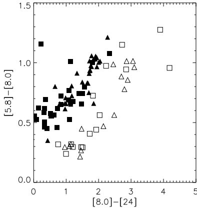
Figure 9. [8]–[24] vs [5.8]–[8.0] colour-colour diagram of AGB stars in the LMC and SMC. Black symbols represent AGB C-rich stars. Open symbols represent AGB O-rich stars. Squares correspond to stars in the SMC and triangles to stars in the LMC.
