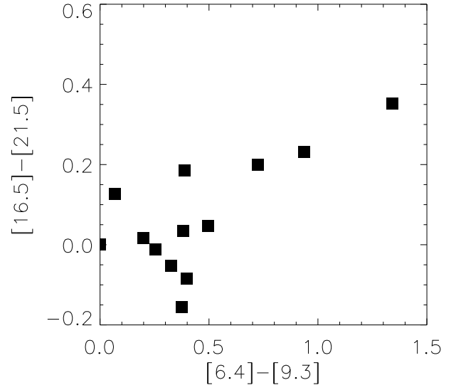
Figure 7. The [6.4]-[9.3] versus [16.5]-[21.5] colour-colour diagram of the stars in our SMC sample.
