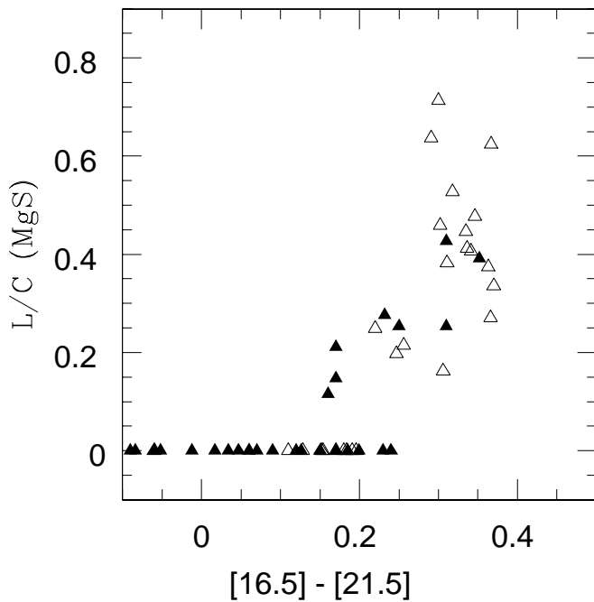
Figure 14. Strength of the MgS feature, versus [16.5] - [21.5] colour. Filled triangles: SMC stars (present sample and Sloan et al. 2006); open triangles: LMC stars (Zijlstra et al. 2006). The band strength is defined as the integrated line-to-continuum ratio (Sect. 6).
