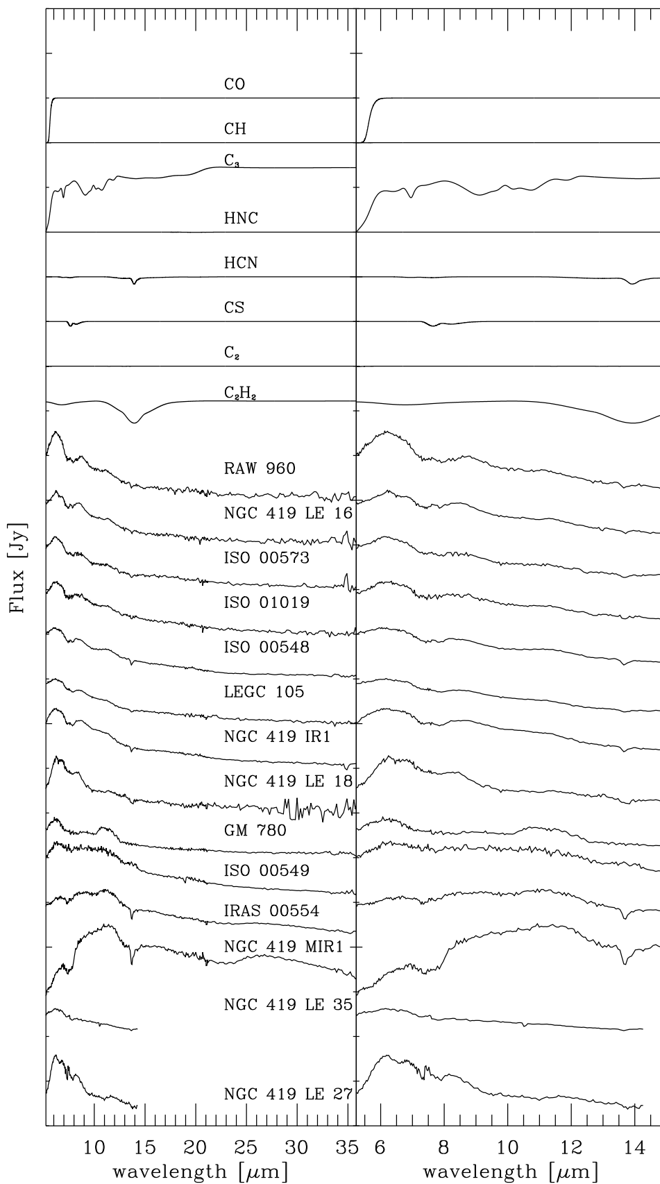
Figure 3. Spectra of the carbon-rich stars observed in the SMC. The two stars at the bottom have been observed only in SL. All other stars are ordered by dust temperature. Blue stars are at the top and red ones at the bottom. Molecular templates are shown at the top (see Sect. 4.3).
