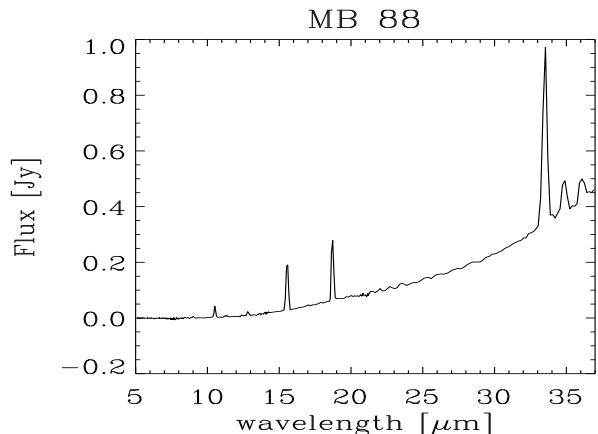
Figure 4. Spectrum of the red object MB 88. This object shows emission lines and could be associated with an HII region. Emission lines from SiV (10.51 \mu m), NeII (12.81 \mu m), SiIII (18.71 and 33.48 \mu m), SiII (34.83 \mu m) and NeIII (35.97 \mu m) are observed.
