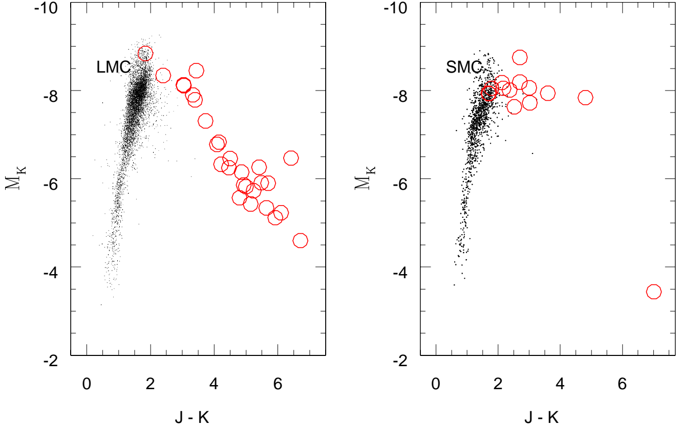
Figure 2. The M_K , J-K diagram for all known optical carbon stars in the LMC and SMC. Samples are taken from Kontizas et al. (2001) and Rebeiro et al. (1993); infrared magnitudes are from 2MASS. Open circles show the Spitzer targets discussed in Zijlstra et al. (2006) and in this paper. LMC photometry for these is from Groenewegen et al. (2007); where no J is available, we assumed J-K \sim 0.6 + 1.84 \times (H-K) . The J-K \approx 7 for NGC418 MIR1 was estimated from its K-L colour.
