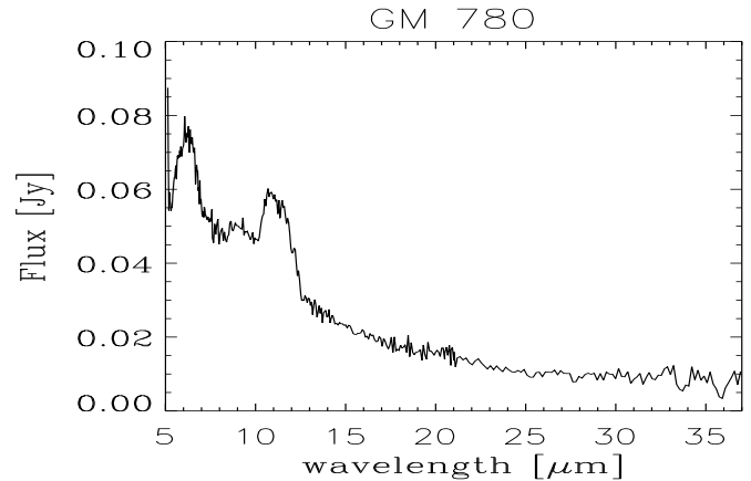
Figure 8. The peculiar spectrum of GM 780.
