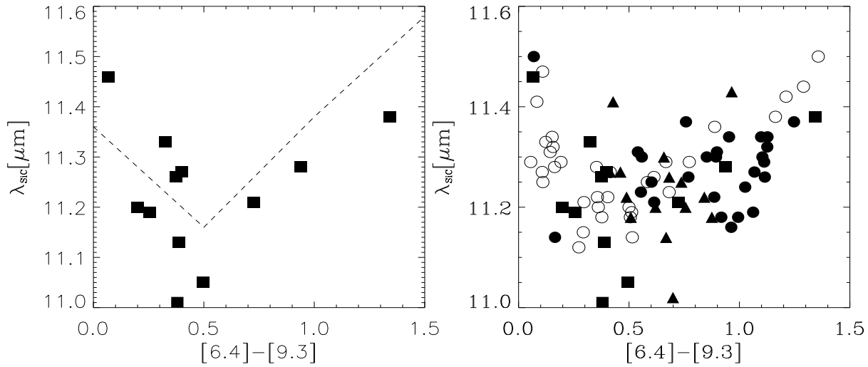
Figure 13. Apparent central wavelength of the SiC feature as a function of the [6.4] - [9.3] colour. Left panel: our SMC sample. Right panel: filled squares represent our SMC sample, triangles Sloan et al. (SMC), open circles Sloan et al. (Galactic) sample and filled circles Zijlstra et al. (LMC). The dashed line is the fit for Galactic stars (Sloan et al. 2006).
