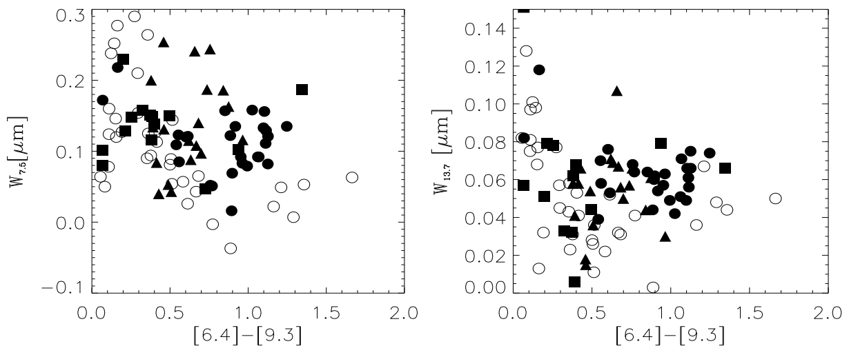
Figure 16. The equivalent width of the C_2H_2 band at 7.5\mu m (left) and 13.7\mu m (right) as a function of the [6.4]–[9.3] colour. Filled squares represents our SMC sample, triangles the Sloan et al. SMC sample, open circles the Sloan et al. Galactic sample and filled circles the Zijlstra et al. LMC sample.
