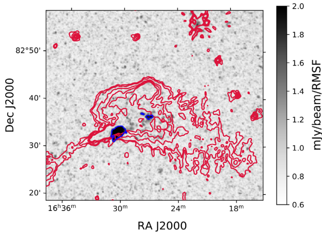
Figure 13. Polarization in the northern lobe of NGC 6251. Grey-scale shows peak polarization in the Faraday depth cube, with blue contours at 8\sigma . Red contours show unpolarized emission in the same LOFAR data at 3, 5, 10, 15, 20 \times \sigma_{\text{rms}} , where \sigma_{\text{rms}} = 2.0 \text{ mJy beam}^{-1} . Faraday spectra for representative pixels in the polarization-detected knot and lobe are shown in Fig. 14.
