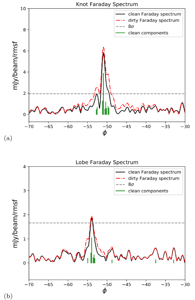
Figure 14. Faraday spectra for pixels in the polarization-detected (a) knot and (b) lobe in Fig. 13. The dirty Faraday spectra are shown as in Fig. 12; also shown are the spectra after cleaning.
