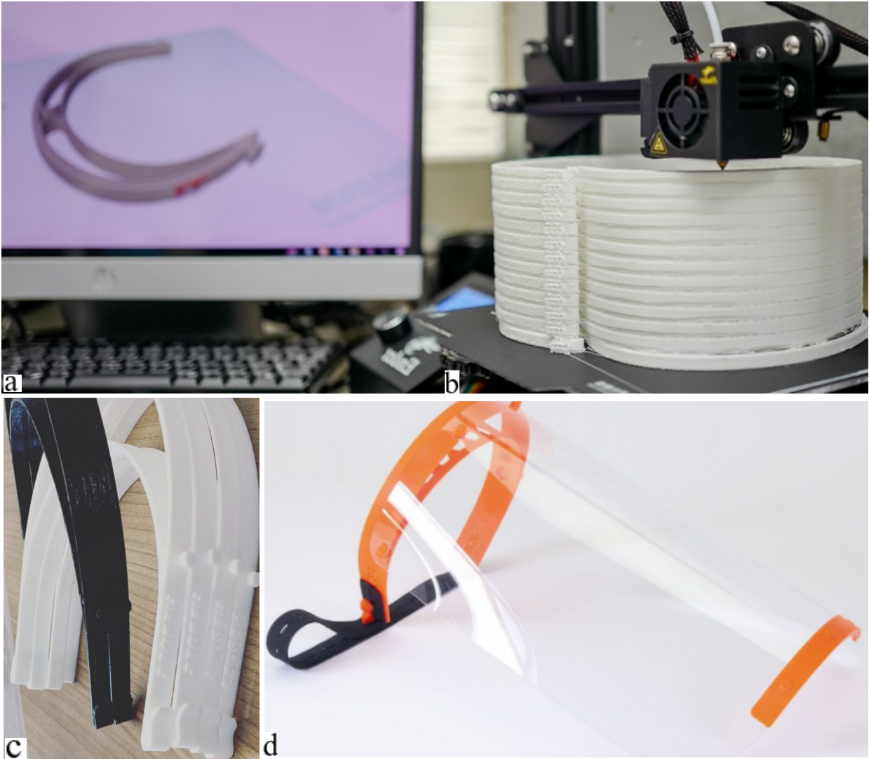
Fig. 7. 3D printing of respiratory face shield using double-sided tape, showing the (a) CAD design, (b) printing process, (c) finish product and (d) complete face shield with films.
