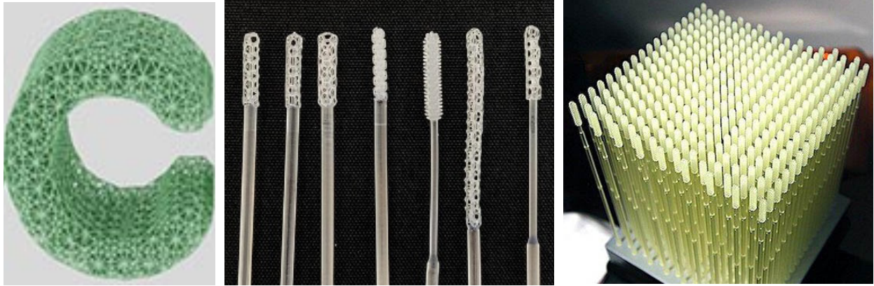
Fig. 6. Lattice structures of the 3D-printed antibacterial bio-cellulose swabs produced for the COVID-19 test.
