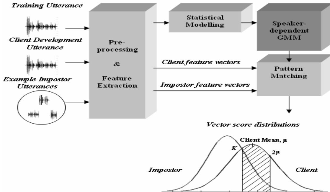
Figure 1. Approach to determining speaker-dependent pruning regions
