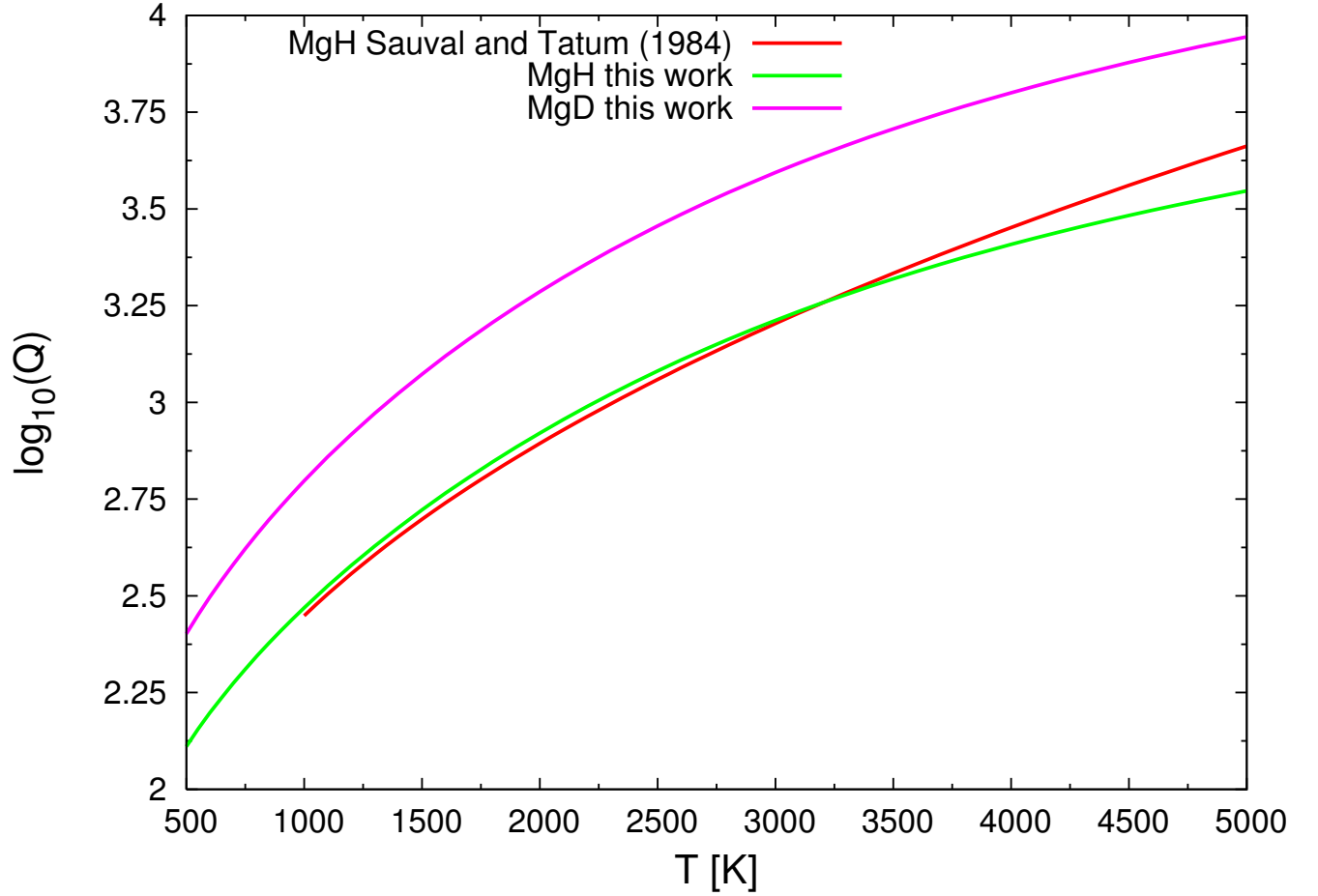
Figure 1. Partition functions of MgH and MgD computed in this work, and the fit of Sauval & Tatum (1984).
