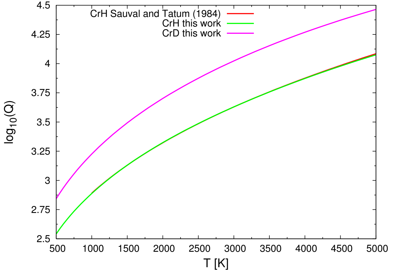
Figure 2. Partition functions of CrH and CrD computed in this work, and the fit of of Sauval and Tatum (1984).
