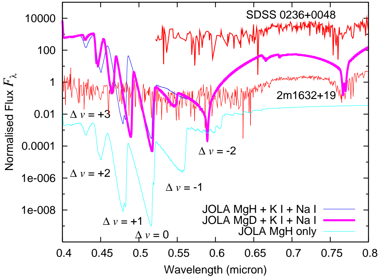
Figure 3. Molecular bands of the A \ ^2\Pi - X \ ^2\Sigma^+ system of MgH and MgD in the theoretical spectrum computed for a 1800/5.0/0 COND model atmosphere. Spectra are shown for D/H = 1 . The lower line on the plot shows the pure spectrum of MgH computed in the framework of JOLA approximation. For comparison the observed spectra of two L dwarfs 2MASS1632+19 (Martín et al. 1999) and SDSS 0236+0048 (Leggett et al. 2001) are shown as solid lines.
