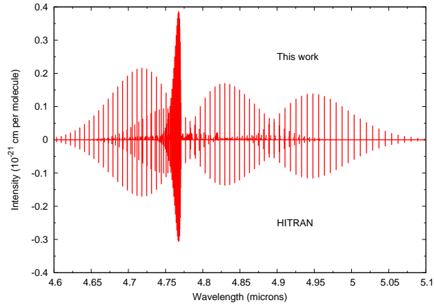
Figure 1. The integrated intensity and frequency of lines of the H^{13}CN v_3 (CN stretch) fundamental and the 3v_2 (bend) overtone at 296 K. The lines from the linelist of this work are shown with positive intensity and lines from the HITRAN database (Rothman et al. 2005) are shown with negatively intensity.
