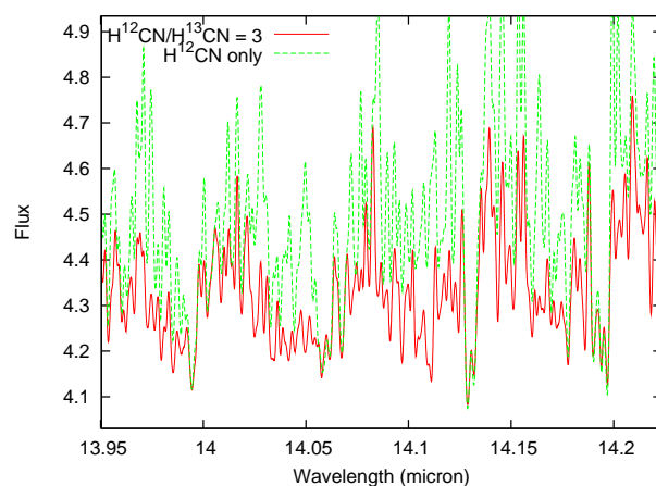
Figure 6. Synthetic spectra computed of WZ Cas computed for the pure H^{12}CN line list (dashed line) and H^{12}CN + H^{13}CN lists. In the last case ^{12}C/^{13}C = 3 was adopted. The spectra are convolved to correspond to a resolution of 10000.
