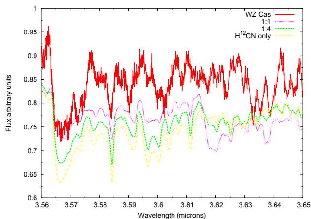
Figure 5. Synthetic and observed spectra for WZ Cas, the synthetic spectra have been displaced from the observed spectrum by 0.06 flux units. The synthetic spectra are shown for H^{13}CN to H^{12}CN ratios of 0, 1/4 and 1.
