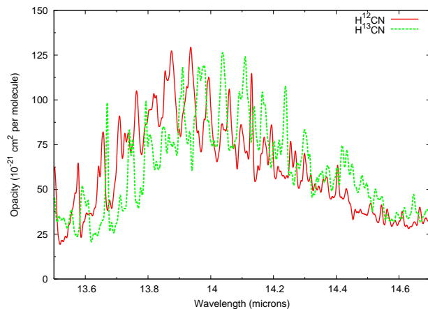
Figure 4. The absorption cross-section per molecule for the \text{H}^{12}\text{CN} and \text{H}^{13}\text{CN} v_2 (bend) fundamental and hot bands at 3000 K.
