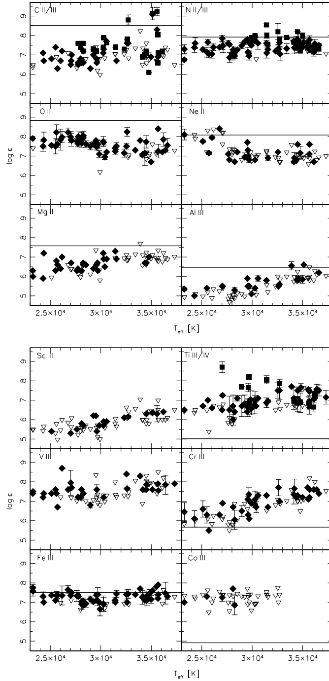
Figure 1. The abundances of selected elements are plotted against the effective temperature. If two ionization stages are present, the lower one is marked by diamonds, the higher one by rectangles. Open triangles mark upper limits. Solar abundances (Grevesse & Sauval 1998) are drawn as horizontal lines. The solar abundances of scandium ( \log \epsilon_{\text{Sc}} = 3.17 ) and vanadium ( \log \epsilon_{\text{V}} = 4.00 ) are below the plotted range.
