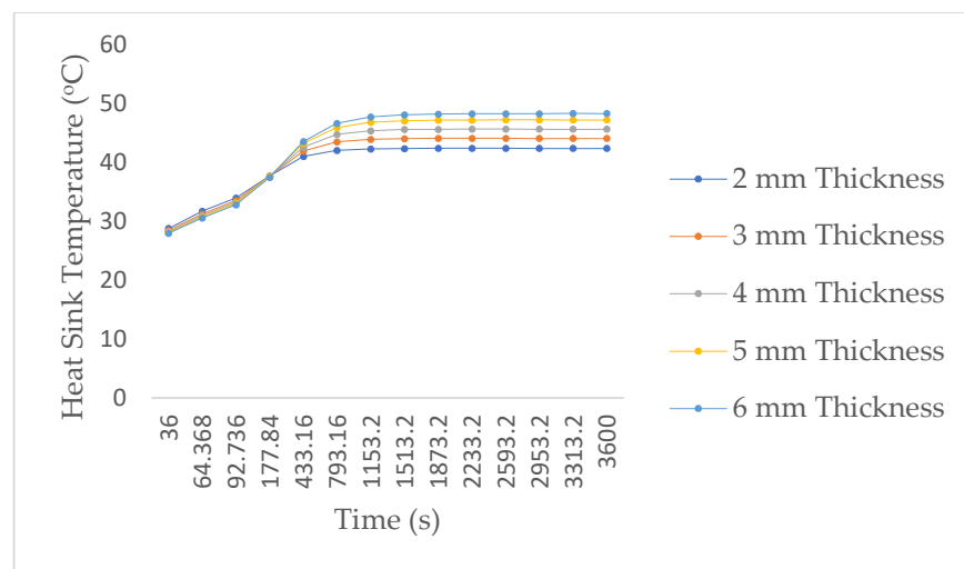
Figure 5. Temperature plot of heat sink at 9.7 W.
