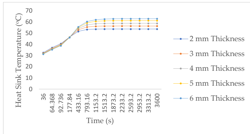
Figure 6. Temperature plot of heat sink at 15.03 W.
