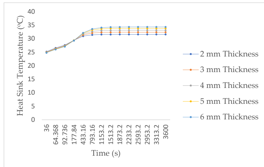
Figure 4. Temperature plot of heat sink at 4.55 W.
