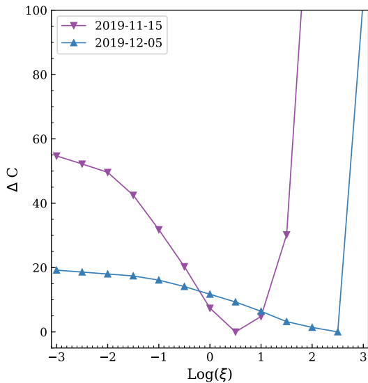
Fig. 6. Change in C -statistics ( \Delta C ) for models with different ionization parameters for the X-ray obscurer. These are obtained by varying the ionization parameter of the obscurer (frozen to different values) of Models M1 in Tables 2 and 3 and re-fitting the observed 2019 spectra.
