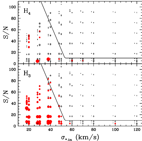
Figure 4. Reliability of the h_3 and h_4 measurements from Monte Carlo simulations. Upper panel: The value of |\Delta h_4| obtained for h_3 = 0 as a function of \sigma_{*,in} and S/N . The values obtained for h_4 = 0 are shifted from those obtained with h_4 = -0.1 for viewing convenience. Symbol size is proportional to the measured value. Open and filled symbols correspond to |\Delta h_4| smaller and larger than 0.1, respectively. The minimum S/N ratios to obtain reliable measurements of h_4 for the different \sigma_{*,in} are connected with a continuous line. Lower panel: As in the upper panel but for |\Delta h_3| .
