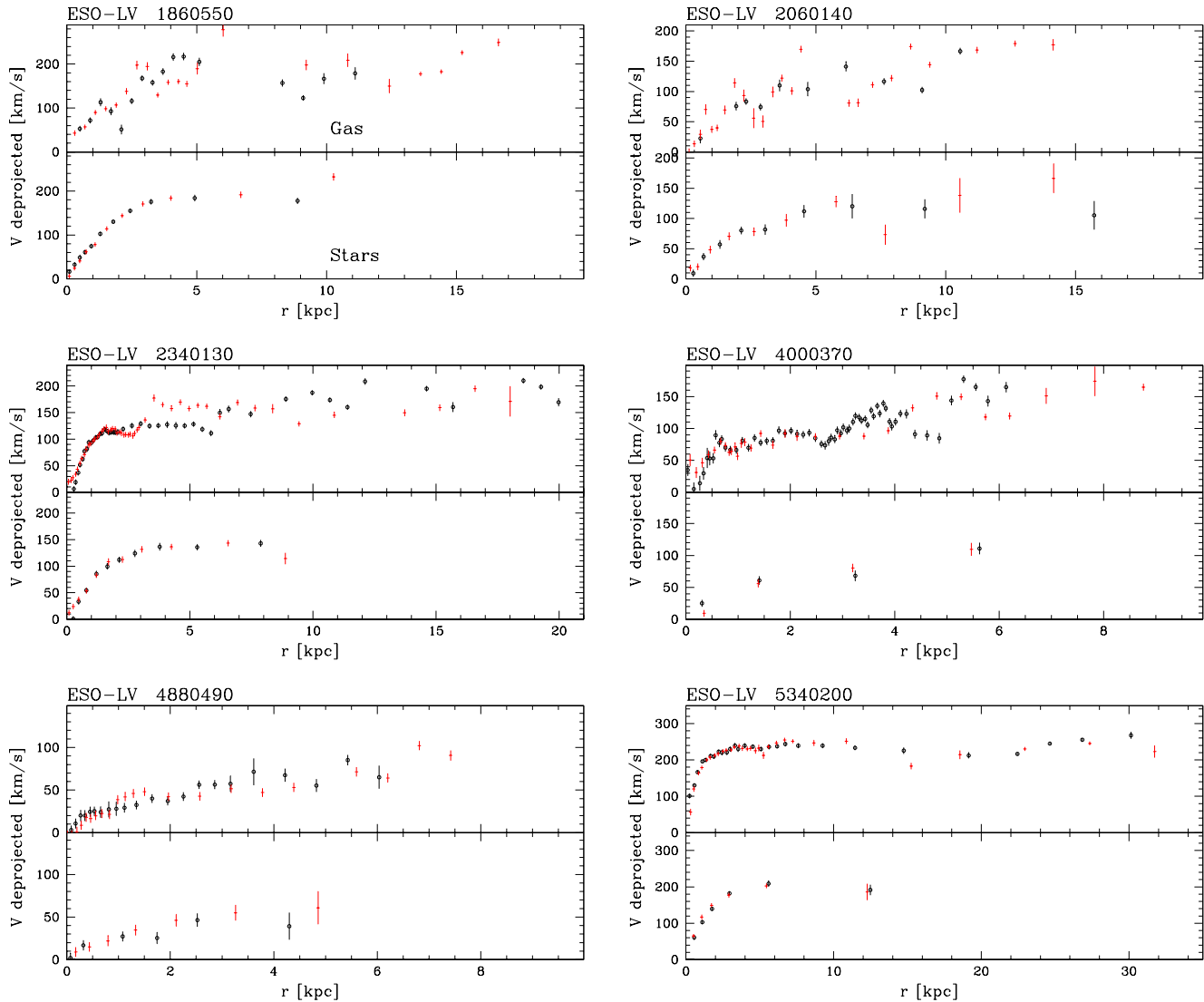
Figure 8. Ionized-gas and stellar rotation curves of the sample galaxies. The velocities of the ionized gas (upper panel) and stellar component (lower panel) are shown after being folded around the symmetry centre and deprojected by taking into account the disc inclination and the misalignment between the observed axis and the galaxy major axis.
