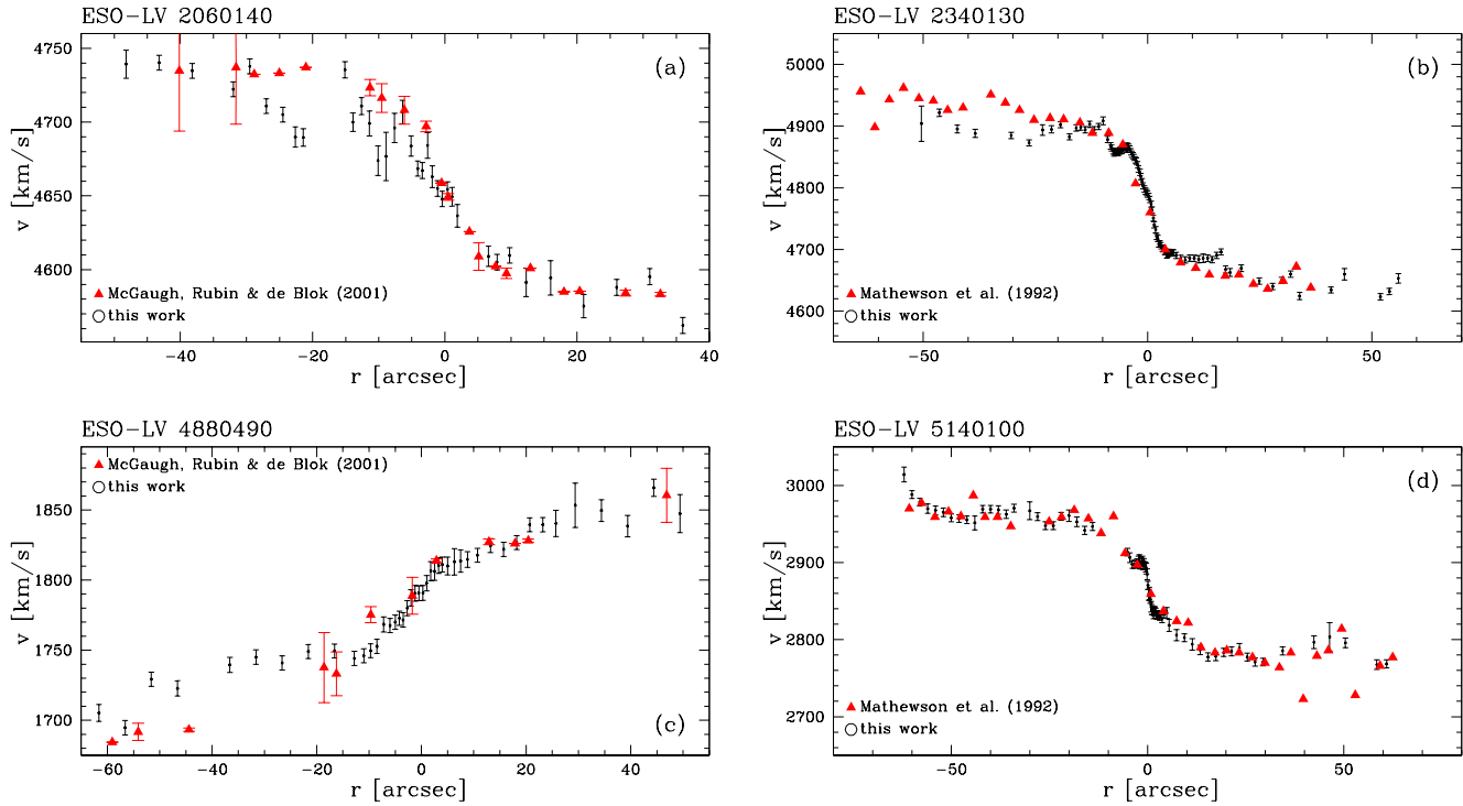
Figure 7. The line-of-sight velocities of the ionized gas derived in this study (circles) for ESO-LV 2060140, ESO-LV 2340130, ESO-LV 4880490, and ESO-LV 5140100 [see App. A] compared with those (triangles) obtained by Mathewson et al. (1992) and McGaugh et al. (2001).
