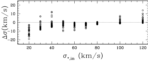
Figure 5. Reliability of \sigma_* measurements from Monte Carlo simulations. The values of \Delta\sigma_* is plotted as a function of \sigma_* only for the artificial spectra with reliable measurements of h_3 and h_4 .
