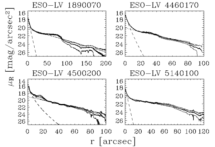
Figure A1. As in Fig. 1 but for the HSB galaxies.
