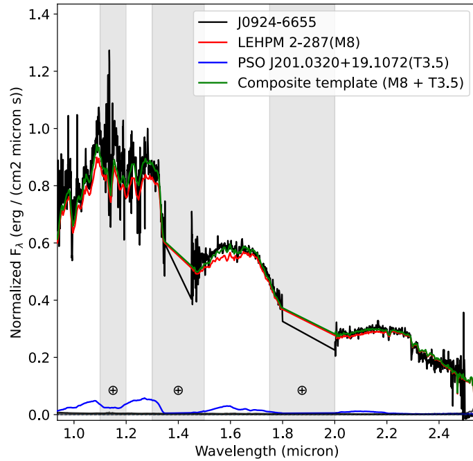
Fig. B.2. Spectrum of J0924-6655 and template spectra of its component, a M8 (red) and a T3.5 (blue), as well as their composite template (green).
