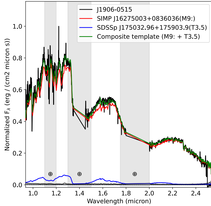
Fig. B.1. Spectrum of J1906-0515 and template spectra of its component, a M9 (red) and a T3.5 (blue), as well as their composite template (green).
