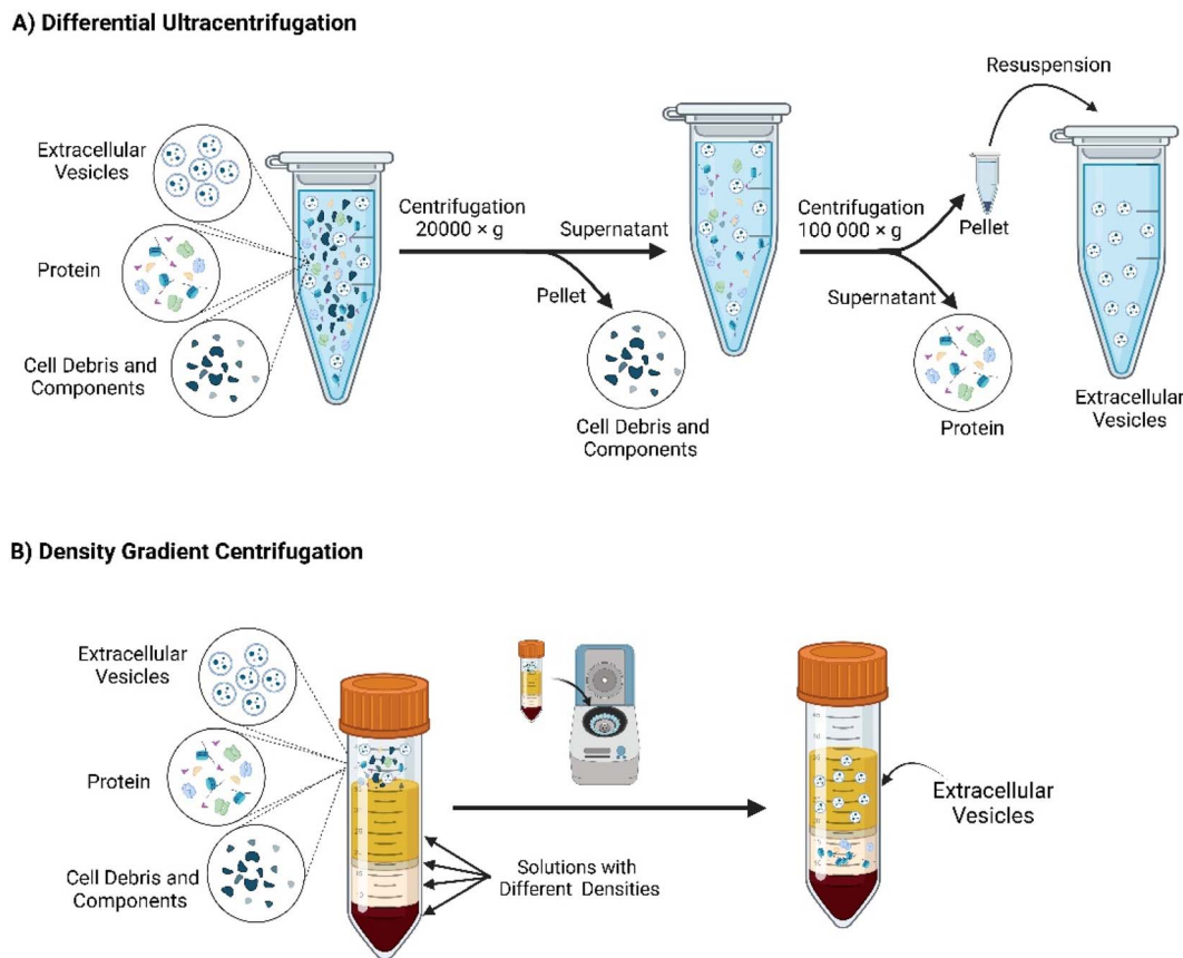
Fig. 2 Isolation of extracellular vesicles using density-based methods (A) differential ultracentrifugation in a two-step manner to eliminate cell debris and proteins, (B) density gradient centrifugation using pre-loaded centrifugal tubes.
