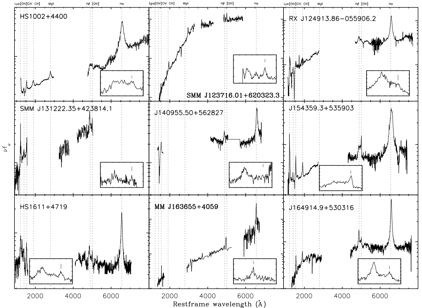
Figure 2. Restframe UV–near-infrared spectra for our sample of submm-detected QSOs. The insets show the region around the H \beta and [OIII] \lambda 5007 emission lines (all insets cover the wavelength range 4675–5100Å), except in the case of J163655, and the redshifts derived from the [OIII] \lambda 5007 emission are indicated. The redshift for J163655 was taken from the redshifted H \alpha due to ambiguity in the [OIII] \lambda 5007 emission lying near the edge of the wavelength coverage of the spectrograph; the inset therefore shows the region around H \alpha . The region around 5100–5500Å in J1409 has been masked due to strong atmospheric absorption.
