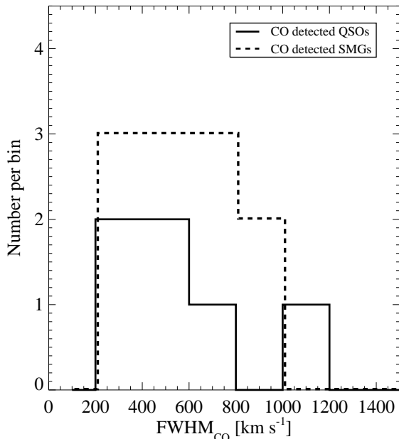
Figure 8. Comparison of the distributions of CO FWHM for 11 SMGs and 6 QSO with detected CO emission. The distributions have medians of (530 \pm 110) \text{ km s}^{-1} (for a mix of single and double Gaussian profile fits), and (550 \pm 180) \text{ km s}^{-1} for SMGs and QSOs, respectively. A KS test reveals a 95% probability that the SMG and QSO CO FWHM distributions are drawn from the same parent population (see text). The histograms have been offset slightly for clarity.
