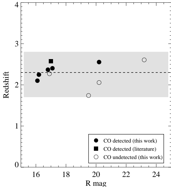
Figure 1. R -band apparent magnitude versus redshift for our sample of submm-detected QSOs. We show that these lie within the interquartile range (shaded region) of the redshift distribution of SMGs (median \langle z \rangle \simeq 2.3 ; dashed line) from Chapman et al. (2005). This shows that we are probing a wide range in optical luminosities (and potentially a wide range in M_{\text{BH}} ) at the epoch where the QSO and SMG populations peak.
