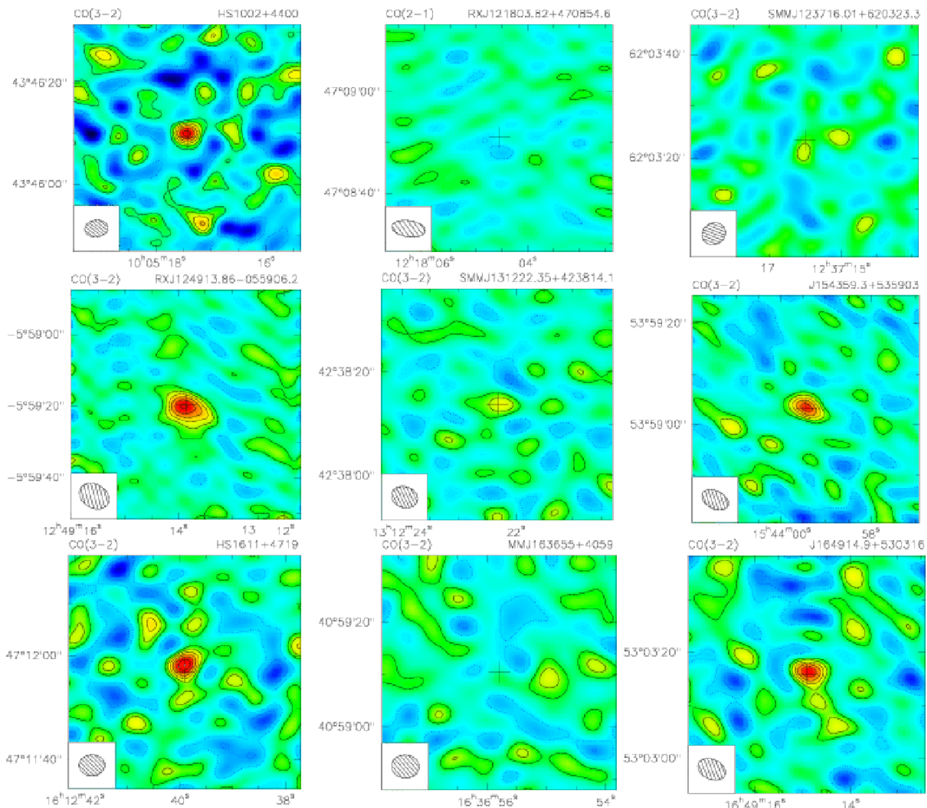
Figure 3. The velocity-integrated mm emission of our nine new submm-detected QSOs. The solid contours are 1, 2, 3... \times \sigma (dashed lines represent equivalent negative contours), where \sigma refers to the noise in each velocity-integrated map (integrated over the width of the CO line) determined by summing over the weights and includes a contribution from the phase noise visibilities. These are the dirty maps (except for RXJ124913.86 which has been cleaned for presentation here to remove significant sidelobe structure) and the synthesized PdBI beams are shown in the insets as hatched ellipses for reference. Crosses indicate the radio or optical position of each source. Detections: The CO-detected sources shown here are HS1002, RXJ124913.86, J131222.35, J154359.3, and HS1611. Note that the CO detection of J131222.35 is marginal. J164914.9 shows a strong continuum detection but no CO detection (see §3.1.10). The positional uncertainties are \simeq 0.5, 0.6, 0.9, 0.7, 0.6 and 0.5 , respectively, for the CO or continuum detected sources (ranked in RA) based on the S/N of the detections and the beam sizes (see text). Non-detections: The three CO and continuum non-detections are shown for comparison and show the 3 mm emission over the central 500 \text{ km s}^{-1} of the spectra (the average line width of our sample).
