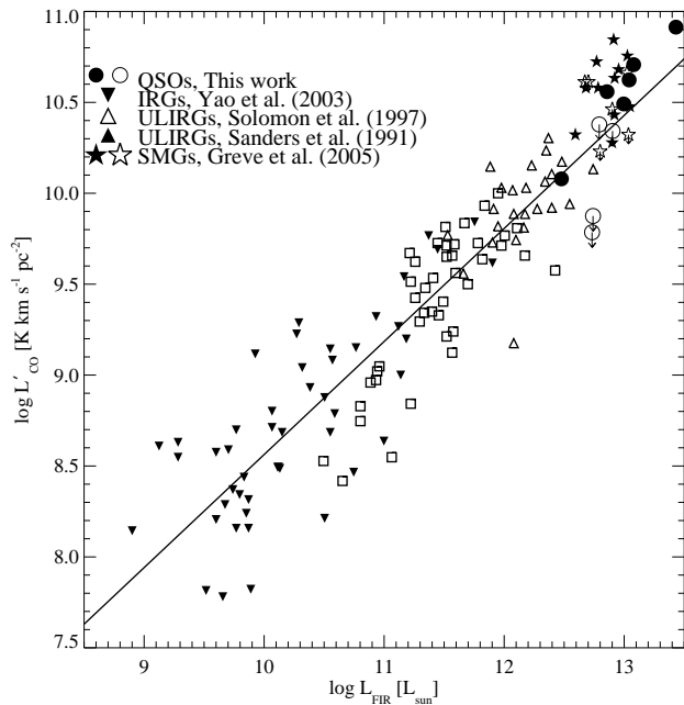
Figure 7. Comparison of the CO and far-infrared luminosities for QSOs, LIRGs, ULIRGs, and SMGs. The line is the best-fitting relation with a form of \log L_{\text{CO}} = \alpha \log L_{\text{FIR}} + \beta to the LIRGs, ULIRGs and SMGs from Greve et al. (2005). The CO-observed ULIRGs and QSOs appear to occupy the same part of the diagram (filled circles/stars represent CO-detections and open circles/stars are CO-nondetections), and lie just above the relation though the offset is not significant given the large errors in L_{\text{FIR}} . This is a particularly useful diagnostic, since it does not depend on the CO-to-gas conversion factor.
