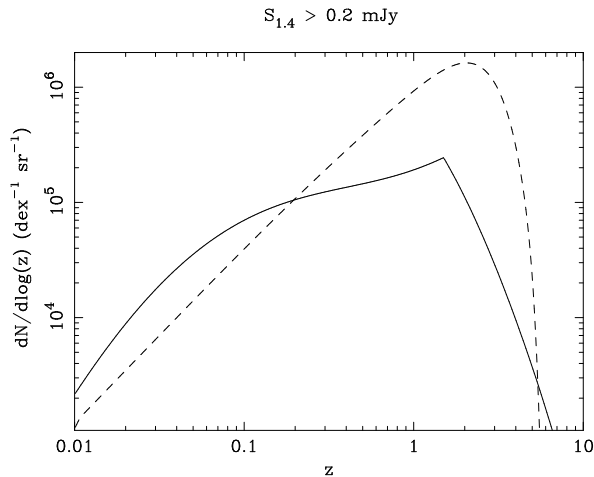
Figure 6. Model redshift distribution for flux limit of 0.2 mJy. The solid and dashed lines denote the starbursts and AGN, respectively.
