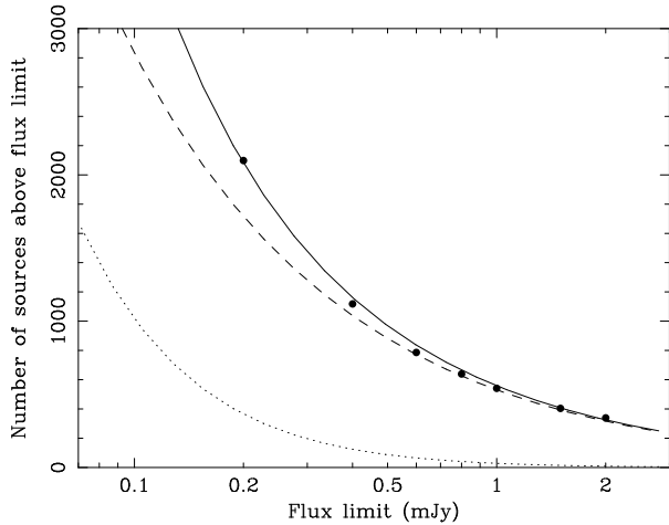
Figure 5. The points show the integral source counts in the central 5.32 \text{ deg}^2 of The Bootes Deep Field where the catalogue is complete down to 0.2 mJy. The dashed and dotted lines show the contributions of the AGN and the starbursts, respectively, and the solid line their sum. The \sqrt{N} error bars are smaller than the symbols. See the text for details.
