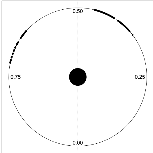
Figure 2. Orbital phase diagram for HD 179949b. Phase 0.00 corresponds to the time of inferior conjunction. The large filled circle at centre represents HD 179949 while the small filled circles represent the phases of observations.
