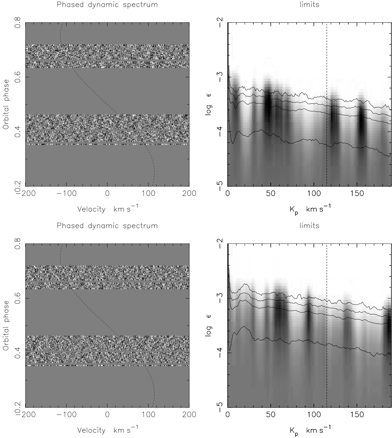
Figure 3. Left: Phased timeseries of the deconvolved residual spectra of HD 179949. The dashed sinusoidal curve represents the expected motion of a planetary signal based on the most probable velocity amplitude, \hat{K}_p = 115 \text{ km s}^{-1} . For plotting purposes, all deconvolved profiles have been normalised to the same noise level to optimise the visible information content of the plot. Right: Relative probability \chi^2 map of planet-star flux ratio \log_{10} \epsilon_0 vs K_p . The first 4 principal components have been subtracted from the timeseries spectra. The greyscale in the probability maps represents the probability relative to the best fitting model in the range white for 0 to black for 1. Numerous enhancements in \chi^2 result from low level systematic residuals (see main text) which can not effectively be removed. Plotted are the 68.3, 95.4, 99 and 99.9 per cent (bottom to top) confidence levels for a planetary signal detection. No planetary signal is detected at the most probable velocity amplitude, \hat{K}_p , which is represented by the vertical dashed line.
