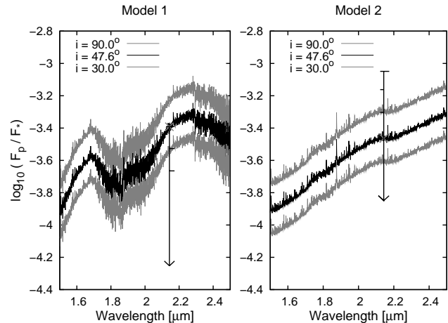
Figure 4. Model and 2.14 \mu\text{m} planet/Star flux ratios for HD 179949b. Shown are models for model 1, absorption (left) and model 2, TiO/VO stratosphere, emission spectrum (right). Some apparent emission features are due to stellar absorption lines and result from dividing the planet spectrum by the stellar spectrum. The black crosses indicate the mean model flux over the wavelength of observations for the most probable inclination. Upper limits corresponding to the levels in Fig. 3 (99.9, 99 and 95.4 per cent) are marked by horizontal bars (from top to bottom) for our analysis using each model. The 99.9 per cent observational upper limit is coincident with the mean flux level for the model 1 model. The width of the top horizontal bar in each case (99.9 per cent confidence) represents the wavelength range of the CRRES spectroscopic observations. For model 1, we can marginally exclude the model with 99.9 per cent confidence at the most probable inclination of 47.6°. For model 2 we are unable to exclude the model since the 95.4 per cent confidence level ( 2\text{-}\sigma ) is above the model flux ratio and artifacts are present between 2\text{-}\sigma and 1\text{-}\sigma (68.3 per cent confidence marked by the arrow).
