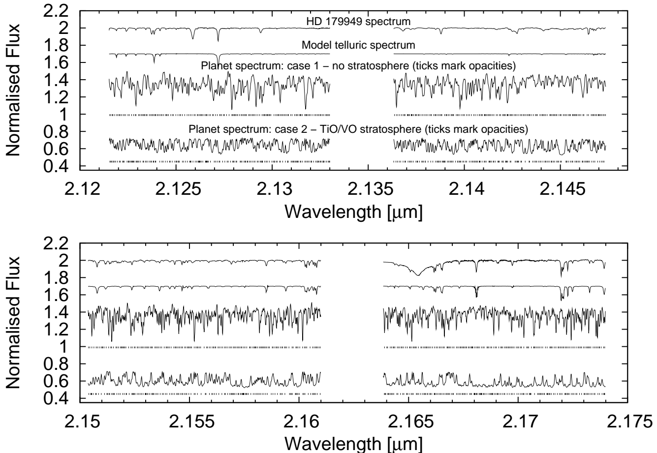
Figure 1. CRiRES wavelength coverage of HD 179949. The four segments (left to right and top to bottom) are the spectral regions recorded on detectors 1-4 respectively. Plotted (top to bottom) in each panel are the mean spectrum for 2007 July 26, model telluric spectrum, model planet spectrum with TiO/VO removed (model 1) and model planet spectrum with TiO/VO stratosphere (model 2). For model 2, the transitions are in emission and are weaker relative to the normalised continuum in the 2.120 \mu\text{m} –2.174 \mu\text{m} spectral window. The model spectra have been convolved with a Gaussian to match the instrumental resolution. The tick marks represent opacity wavelengths (before convolution) for each planetary model.
