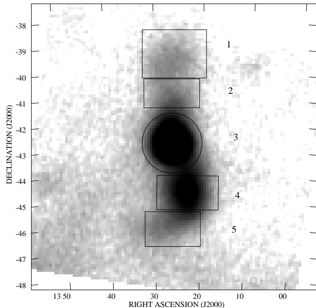
Figure 3. Regions for the spectral extractions whose results are listed in Table 1 and plotted in Fig. 4. The greyscale shows the 20-GHz WMAP data.
