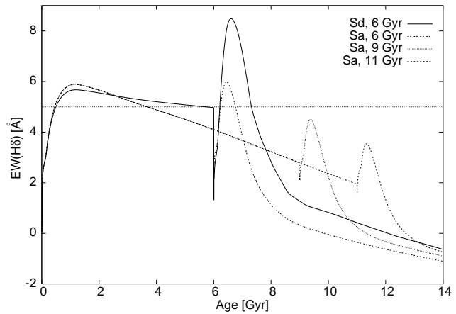
Figure 5. Time evolution of \text{EW}(H\delta) in galaxies with different burst scenarios (Sa, burst of 70% at 6 Gyr, decline time 0.1 Gyr; Sd, burst of 70% at 6 Gyr, decline time 0.1 Gyr; Sa, burst of 70% at 11 Gyr, decline time 0.1 Gyr).
