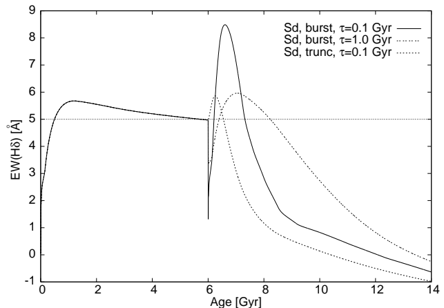
Figure 6. Time evolution of \text{EW}(H\delta) in galaxies with different burst scenarios (Sd, burst of 70% at 6 Gyr, decline time 0.1 Gyr; Sd, burst of 70% at 6 Gyr, decline time 1.0 Gyr; Sd, truncation at 6 Gyr, decline time 0.1 Gyr).
