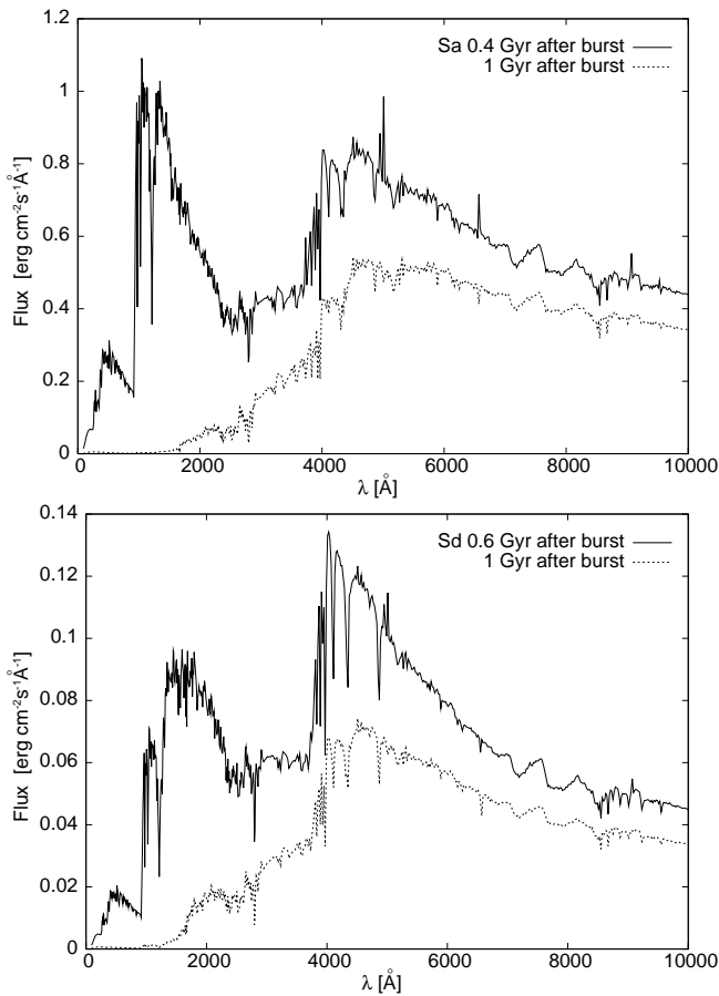
Figure 12. Spectra of an Sa model (burst 50%) and an Sd model (burst 70%) in the burst (at 6 Gyr, decline times 0.1 Gyr). The spectra show the galaxies in their post-starburst phase at their maximum EW( H\delta ) and 1 Gyr after the burst.
