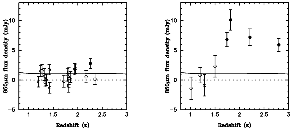
FIG. 2.— Left : 850 \mu\text{m} flux densities of the sample of 20 X-ray-unabsorbed QSOs. Right : 850 \mu\text{m} flux densities of the matched sample of X-ray-absorbed QSOs, adapted from Page et al. (2001a). In both panels, sources that are detected at greater than 3\sigma confidence are plotted as filled circles, while nondetections are shown as open circles. The solid line on both panels shows the predicted 850 \mu\text{m} flux density of the nearby submillimeter luminous, X-ray-absorbed QSO Mrk 231 if it were viewed at redshift z .
