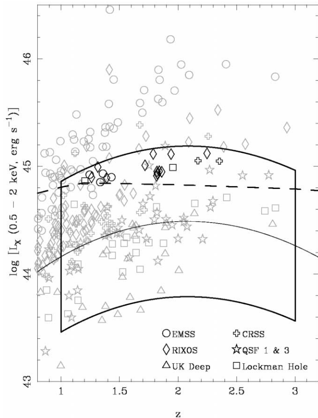
FIG. 1.—Selection of the sample. The data points show the redshifts and X-ray luminosities of X-ray–selected AGNs from a number of surveys with different flux limits and sky areas. The thin solid line shows the position of \log L_* as a function of redshift assuming the best-fit model luminosity function from Page et al. (1997), and the thick solid line encloses the region ( 1 < z < 3 , \log L_* - 0.7 < \log L < \log L_* + 0.7 ), in which the majority of AGN comoving luminosity density is produced. The bold dashed line is the limit at which sources are expected to have a flux of 3 mJy at 850 \mu\text{m} if they have star formation–powered far-infrared (FIR) luminosities equal to their AGN bolometric luminosities, and assuming FIR spectra similar to that of Mrk 231. The AGNs above the dashed line but within the region enclosed by the thick line are the objects that can be usefully probed with SCUBA and are relevant to the production of the universe’s accretion luminosity. Sources selected for submillimeter observations are shown in black rather than gray.
