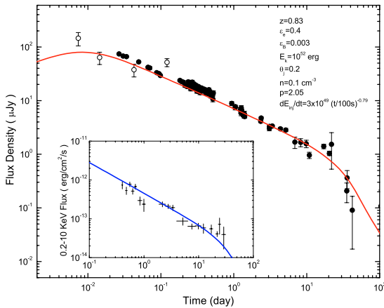
Fig. 7. Modeling R -band (host subtracted) and X-ray (inset) afterglow lightcurves of XRF 050824 with continuous energy injection. The fitting parameters are given in the figure and are further discussed in the text.
