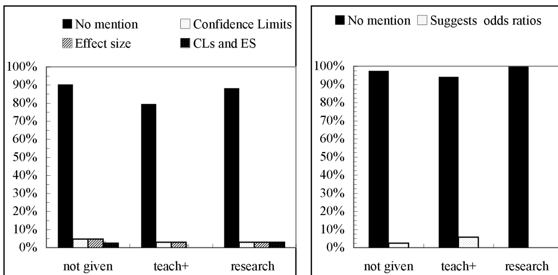
Figure 2. Reports of effect sizes/confidence interval (left panel) and odds ratios (right panel)
