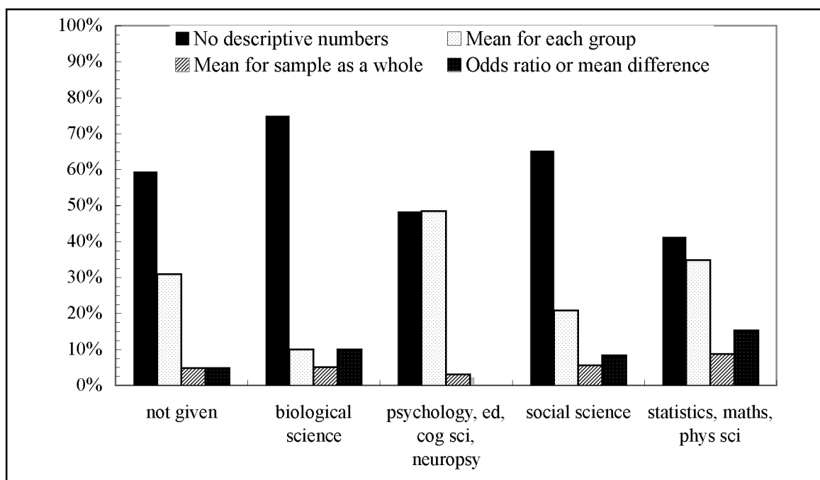
Figure 1. Percentage choices of descriptive statistics reporting as a function of discipline.
