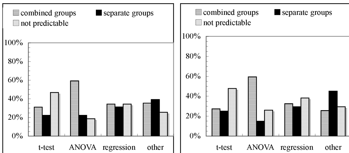
Figure 3. The effect of most frequent analysis on predictions of replications. Scenario 1, left panel; scenario 2, right panel.
