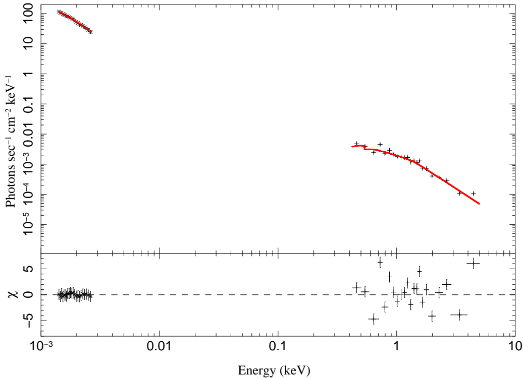
Figure 6. The SED of the optical 300V spectrum (×) and the X-ray spectrum (+), at 66 min after the burst. The solid line shows the best fitting model, a broken power law with spectral slopes \beta_{\text{X}} = 1.59 \pm 0.11 and \beta_{\text{opt}} = 0.71 \pm 0.02 , for an SMC-type dust extinction, see Table 4. The residuals are displayed in the bottom panel.
