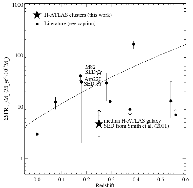
Figure 4. Measures of the mass-normalised SFRs in galaxy clusters out to z \sim 0.6 , adapted from fig. 6 of Geach et al. (2006). The SFRs are derived from the mid- or far-infrared populations within \sim 2 Mpc and are normalised to the best estimate of the total (luminous+dark) cluster mass. Listed in order of increasing redshift, they are: Perseus (Meusinger et al. 2000), A3112 (Braglia et al. 2011), A2218 (Biviano et al. 2004), A1689 (Fadda et al. 2000; Duc et al. 2002), H-ATLAS (this work), A1758 (Haines et al. 2009), the Bullet cluster (Rawle et al. 2010; Clowe, Gonzalez & Markevitch 2004; Markevitch 2006), A370 (Metcalfe, Fadda & Biviano 2005), Cl 0024+16 and MS0451–03 (Geach et al. 2006), and J1888.16LC (Duc et al. 2004). An evolutionary model for the counts of star-forming ULIRGs from Cowie et al. (2004) is overlaid as a guide only, and has been normalised arbitrarily to the mean star formation rate in Cl 0024+16 and MS 0451–03 from Geach et al. (2006). This plot shows an increasing rate of activity in more distant clusters as traced through their mid- or far-infrared populations, albeit with a large scatter, suggestive that the infrared is a sensitive tracer of environmental changes within the clusters. Note that there are large systematic effects on the points in this plot, with the inferred SFR dependent on the assumed form of the SED, and estimate of the total cluster mass. Given the large uncertainties on the H-ATLAS cluster masses and the cool SED we have adopted, we consider our point a lower limit (as indicated by the arrow). We also show how our result changes if we instead assume an M82 or Arp220 SED (open symbols), to facilitate a comparison with the literature results.
