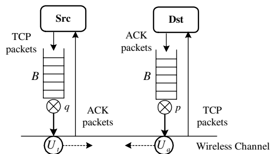
Fig. 2. System model of TCP in wireless adhoc networks
