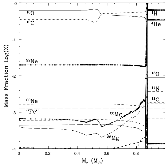
FIGURE 4. Abundances in mass fraction in the inner core of the 6 M_{\odot} star for Y = 0.2775 and Z = 0.02 at the end of the second dredge-up.
