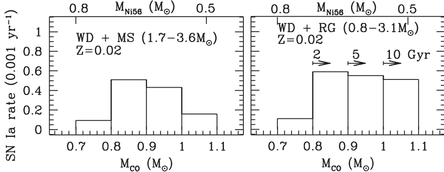
FIGURE 6. SN Ia frequency for a galaxy of mass 2 \times 10^{11} M_{\odot} as a function of M_{CO} for Z=0.02 . For the WD+RG system, constraints from the companion’s age are shown by the arrows. SNe Ia from the WD+MS system occur in spirals but not in ellipticals because of the age effect. M_{CO} and M_{Ni56} is assumed to be related as shown here.
