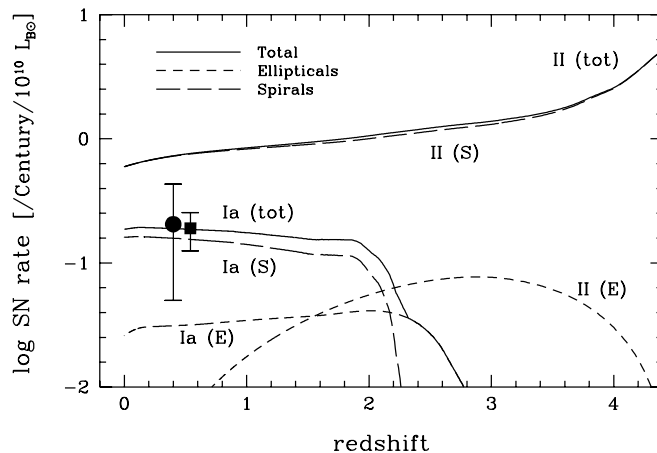
FIGURE 9. The same as Figure 8, but for the formation epochs of ellipticals span at 1 \lesssim z \lesssim 4 , which is corresponding to field ellipticals.
