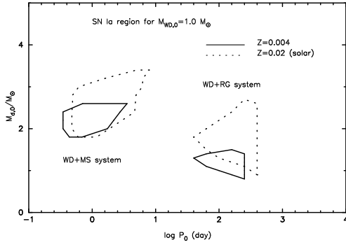
FIGURE 2. The regions of SNe Ia is plotted in the initial orbital period vs. the initial companion mass diagram for the initial WD mass of M_{\text{WD},0} = 1.0M_{\odot} . The dashed and solid lines represent the cases of solar abundance ( Z = 0.02 ) and much lower metallicity of Z = 0.004 , respectively. The left and the right regions correspond to the WD+MS and the WD+RG systems, respectively.
