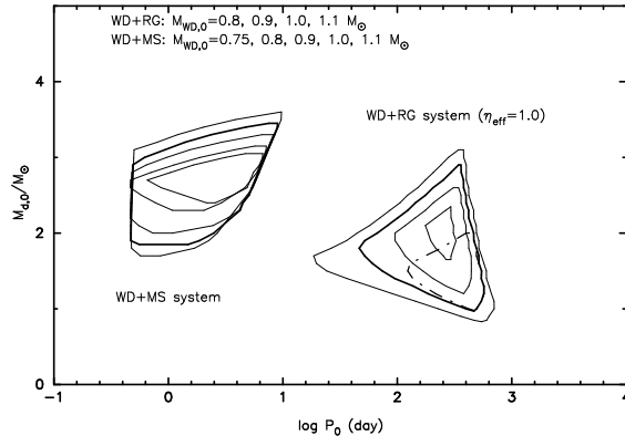
FIGURE 1. The region to produce SNe Ia in the \log P_0 - M_{d,0} plane for five initial WD masses of 0.75M_\odot , 0.8M_\odot , 0.9M_\odot , 1.0M_\odot (heavy solid line), and 1.1M_\odot . The region of M_{WD,0} = 0.7M_\odot almost vanishes for both the WD+MS and WD+RG systems, and the region of M_{WD,0} = 0.75M_\odot vanishes for the WD+RG system. Here, we assume the stripping efficiency of \eta_{\text{eff}} = 1 . For comparison, we show only the region of M_{WD,0} = 1.0M_\odot for a much lower efficiency of \eta_{\text{eff}} = 0.3 by a dash-dotted line.
