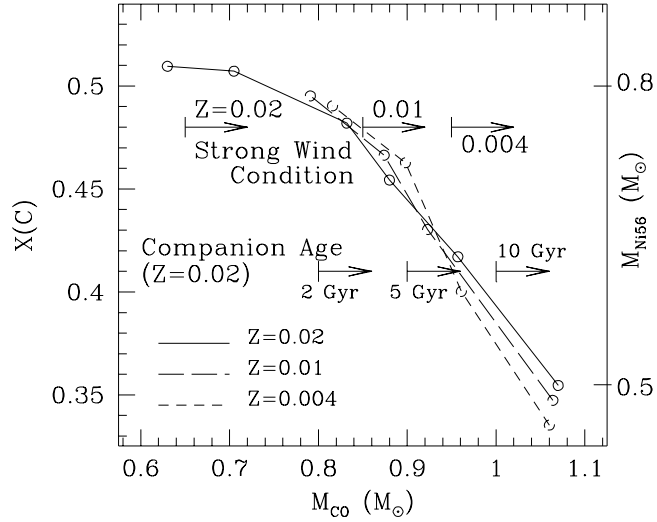
FIGURE 5. The total ^{12}\text{C} mass fraction included in the convective core of mass, M = 1.14M_{\odot} , just before the SN Ia explosion as a function of the C+O core mass before the onset of mass accretion, M_{\text{CO}} . The lower bounds of M_{\text{CO}} obtained from the age effects and the conditions for strong wind to blow are also shown by arrows.
