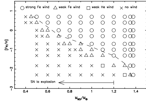
FIGURE 3. WD mass vs. metallicity diagram showing the metallicity dependence of optically thick winds. We regard the wind as “strong” if v_w > v_{\text{esc}} but “weak” if v_w < v_{\text{esc}} . The term of “He” or “Fe” wind denotes that the wind is accelerated by the peak of iron lines near \log T(\text{K}) \sim 5.2 or of helium lines near \log T(\text{K}) \sim 4.6 . The dashed line indicates the demarcation between the “strong” wind and the “weak” wind.
