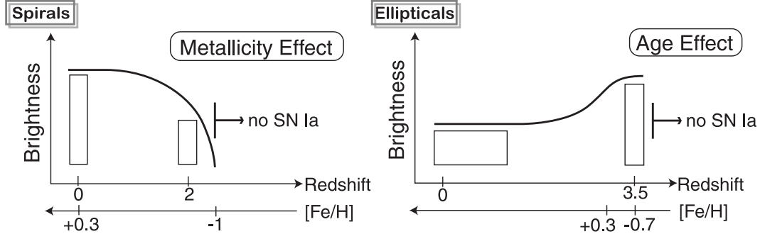
FIGURE 7. Illustration of the predicted variation in SN Ia brightness with redshift.
