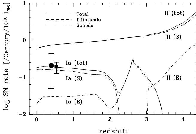
FIGURE 8. The cosmic supernova rates (solid line) as the composite of ellipticals (short-dashed line) and spirals (long-dashed line). The upper three lines show SN II rates, the lower three lines show SN Ia rates. Observational data sources: circle, [63]; square, [10].
