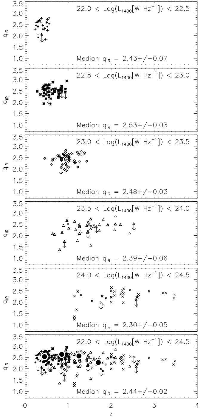
Fig. 3. q_{\text{IR}} versus redshift for our radio-selected galaxies (sample 2), in five bins of K -corrected l_{1.4} , plus the full sample. Values of q_{\text{IR}} for sample 3 are shown (as circles) for comparison.
