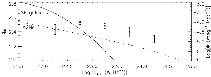
Fig. 4. Median q_{\text{IR}} versus H.4 . The local luminosity functions of starbursts and AGN are shown (Mauch & Sadler 2007).
