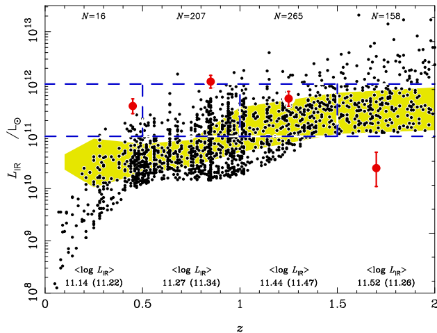
Fig. 5. L_{\text{IR}} (dots; left axis) and q_{\text{IR}} (red circles; right axis) – the former determined via the models of Chary & Elbaz (2001) – versus redshift for our L_{\text{IR}} -matched sample. The luminosity bounds and redshift bins (dashed lines), the number of galaxies in each bin and their predicted (measured) \langle \log L_{\text{IR}} \rangle and measured \langle q_{\text{IR}} \rangle are all shown. The shaded area represents a \pm 1\sigma prediction for q_{\text{IR}} (Swinbank et al. 2008; Ivison et al. 2010).
