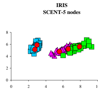
(a) SCENT with 5 leaf nodes
