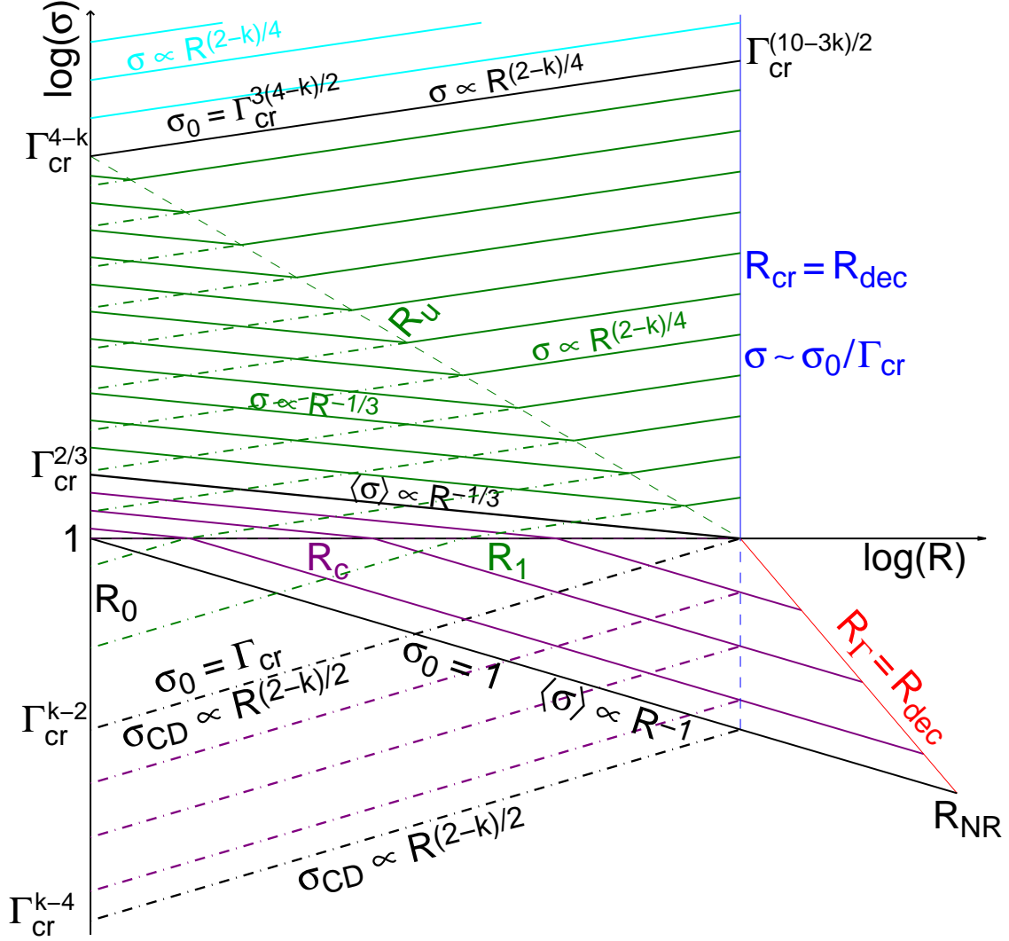
Fig. 6.— The same as Fig. 5 but with the addition of the magnetization just behind the contact discontinuity, \sigma_{CD} (dashed-dotted lines), until it becomes similar to the typical magnetization, \langle \sigma \rangle .
