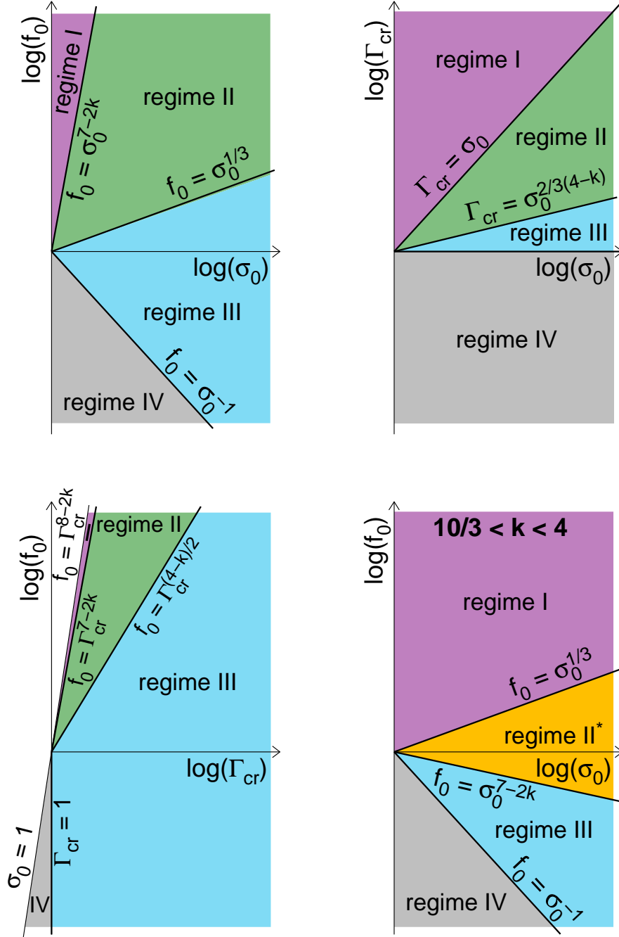
Fig. 10.— Phase space diagrams of the different dynamical regimes: in the f_0 – \sigma_0 plane for k < 10/3 (top left panel), \Gamma_{cr} – \sigma_0 plane for k < 10/3 (top right panel), f_0 – \Gamma_{cr} plane for k < 10/3 (bottom left panel), and in the f_0 – \sigma_0 plane for 10/3 < k < 4 (bottom right panel). Each regime is labeled and denoted by a different color, and the borders between the different regimes are indicated (by labeled thick black lines).
