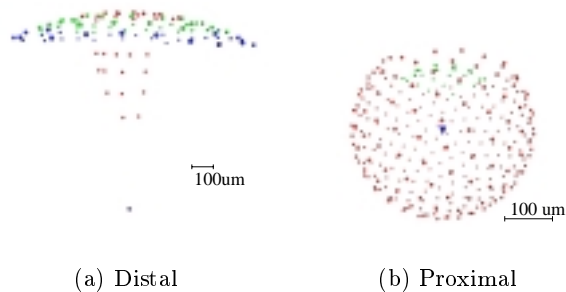
Figure 3: Arrangement of chemical attractants for the 2 developmental environments. The soma of the pyramidal neuron is the lowest object in (a) and the cone at the centre of the sphere of attractants in (b).
