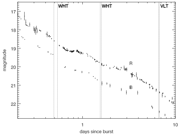
Figure 1. B and R band photometry of GRB 021004 compiled from the literature (Bersier et al. 2003, Fox et al. 2003, Holland et al. 2003, Pandey et al. 2003 and Uemura et al. 2003). The coverage of the WHT and VLT spectra presented here is shown by vertical dotted lines.
