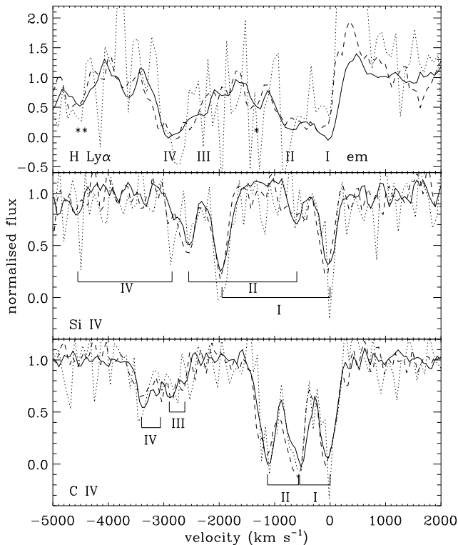
Figure 3. Outflow velocities of the CIV and SiIV absorption doublets (velocities plotted are for the longer wavelength components only) and corresponding hydrogen Ly \alpha systems, divided by the local continua. The solid lines show the WHT observation of 4/10/02, the dashed lines show the WHT observation of 6/10/02 and the dotted lines show the VLT observation of 11/10/02. The 4 velocity systems are denoted by roman numerals, the Ly \alpha emission line (too large in the VLT data to be shown fully on this plot) is labelled ‘em’. Intervening CIV is marked with a * and ** marks the long-wavelength end of the bluest absorption complex.
