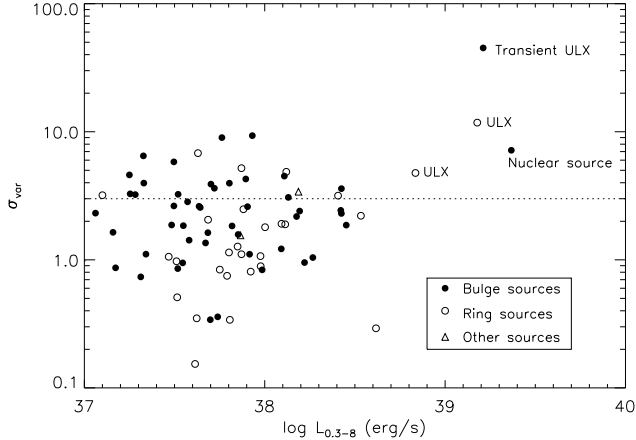
FIG. 7.— Significance of flux variability vs. observed full-band luminosity for the 50 bulge sources (filled dots), 28 ring sources (open dots), and 3 other sources (triangles). Dotted line indicates the > 3\sigma significance level of the flux variability. Note that we calculated flux variability for only sources detected in at least one individual observation; there are insufficient data for variability study of the remaining sources. We studied spectral variability of the few ULX candidates, which show no significant variability in spectral parameters (column density and power-law index).
