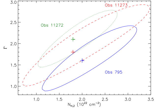
FIG. 6.— 3\sigma confidence contours for the photon index and absorption column density parameters of the nuclear AGN in the three individual observations, observations 795 (blue), 11272 (green), and 11273 (red). The fit parameters in observation 2059 have large uncertainties and is not shown in the plot for clarity. The crosses show the best-fit N_{H,2} and \Gamma values in observations 795, 11272, and 11273, respectively. The larger confidence contour of observation 11273 than that of observation 795 despite of its longer exposure is due to the lower flux/luminosity of the nucleus during this observation. See Section 4.2 for more details. (A color version of this figure is available in the online journal.)
