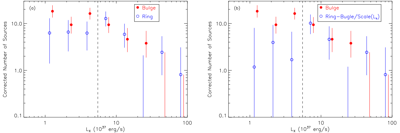
FIG. 11.— Numbers of X-ray sources in given luminosity bins for the bulge, ring [panel (a)], and bulge-subtracted ring [panel (b); see text] populations. The numbers of sources have been corrected for the detection incompleteness and background AGN contamination. The luminosity bins were chosen to be the same for all the populations, and the limiting luminosity is \approx 8.5 \times 10^{36} erg s ^{-1} . The luminosities for the bulge data points were shifted by a small amount for display purpose. For several cases with only error bars and no data points shown in the plot, the numbers of sources are smaller than 0.1. The vertical dashed lines mark the approximate breaks of the XLFs, and are used to separate relatively luminous and relatively faint sources. (A color version of this figure is available in the online journal.)
