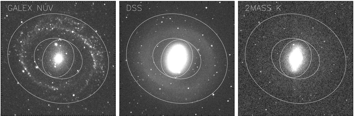
FIG. 1.— Images of NGC 1291 in the GALEX near-UV (NUV, \lambda_{\text{eff}} = 2267 \text{ \AA} ), Digitized Sky Survey red (RG610), and 2MASS K bands. The size of each image is 14' \times 14' , centered on the galactic nucleus. The ellipses outline the bulge and ring regions (see Section 3 for details). The UV ring appears to be dominated by young stars.
