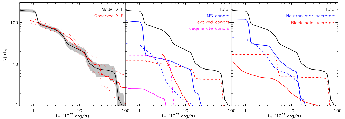
FIG. 10.— Left panel: Synthetic XLF (black solid curve) for the maximum likelihood model. The gray shaded area corresponds to the 1-\sigma error of the XLF due to Poisson statistics and uncertainties in bolometric correction. For comparison the observed combined (corresponding to both the bulge and ring regions) XLF (red solid curve) and the associated 1-\sigma error (red dotted curves) are drawn. Center panel: Contribution of different sub-populations by separating the XRBs into groups of systems with different donor stellar types. Right panel: Contribution of different sub-populations by separating the XRBs into groups with different accretor types. In the center and left panel, solid colored lines denote persistent XRB sub-populations, while dashed colored lines denote transient ones. (A color version of this figure is available in the online journal.)
