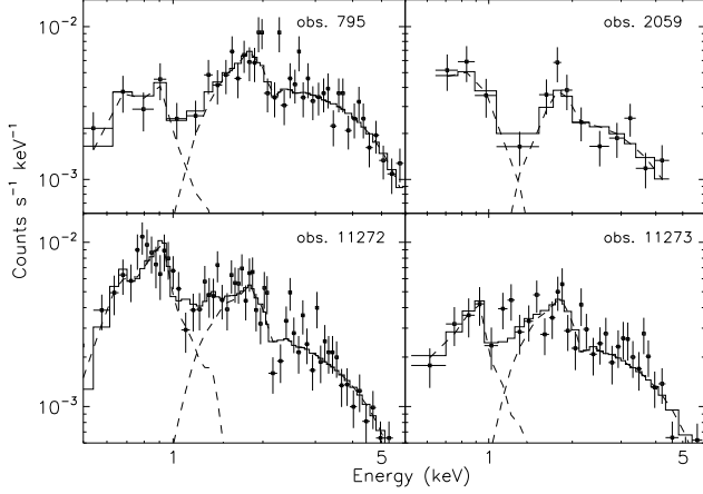
FIG. 5.— X-ray spectra of the nuclear source overlaid with the best-fit models for the four individual observations. The spectra were fit with an absorbed power law plus thermal plasma model (WABS1*APEC+WABS2*POW). The dashed curves show the individual model components. For the thermal component, the temperature (0.15 keV) and column density ( 7.6 \times 10^{21} \text{ cm}^{-2} ) were fixed at the values derived from the stacked spectrum. See Section 4.2 for more details and see Table 3 for the fit parameters.
