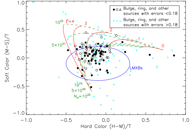
FIG. 8.— X-ray color-color plot for the point sources. S , M , H , and T are the count rates in the 0.3–1.0 keV, 1.0–2.0 keV, 2.0–8.0 keV, and 0.3–8.0 keV bands, respectively. Black data points represent sources with relatively small color errors, while cyan data points represent sources with large errors and are less significant. The green and red tracks show the expected X-ray colors for absorbed power-law spectra with different power-law indices and column densities. The blue ellipse indicates the area that is likely dominated by LMXBs (Prestwich et al. 2003). A significant fraction of the X-ray sources with small color errors are located in the region expected to be dominated by LMXBs. (A color version of this figure is available in the online journal.)
