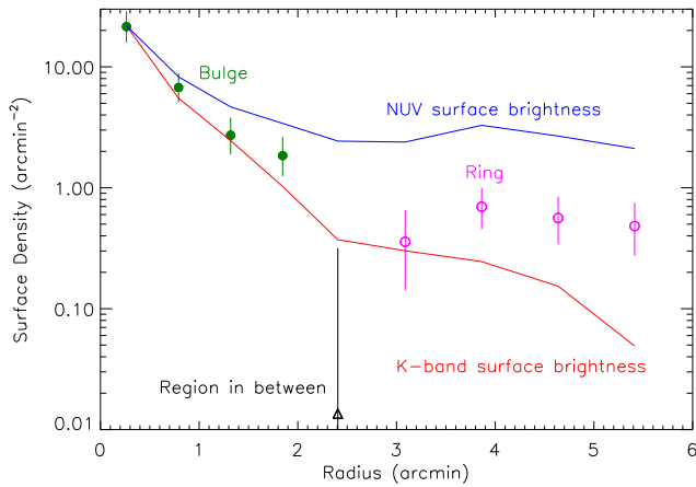
FIG. 4.— Radial profile of the X-ray source surface density. The densities were computed in four elliptical annular regions in the bulge (green filled circles), four elliptical annular regions in the ring (magenta open circles), and one region in between the bulge and the ring (black triangle). The x -axis shows the average distance of each region to the galactic nucleus. The surface densities have been corrected for detection incompleteness and background AGN contamination. Only sources outside the central 10'' -radius region and having L_X > 10^{37} erg s^{-1} are included in the density calculation. The errors of the surface densities were calculated based on the Poisson errors of the number of sources in each bin (Gehrels 1986). The red and blue curves display the surface brightness radial profiles (scaled to the highest X-ray source density) for the GALEX NUV and 2MASS K -band data, respectively. There appears to be an overdensity of X-ray sources in the ring region. (A color version of this figure is available in the online journal.)
