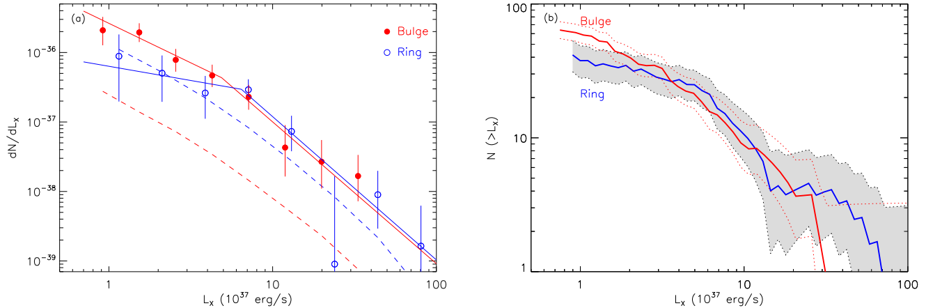
FIG. 9.— Differential [panel (a)] and cumulative [panel (b)] XLFs for the bulge (red filled dots or curve) and ring (blue open dots or curve) populations. The XLFs have been corrected for detection incompleteness and AGN contamination. In panel (a), the dashed curves represent the expected XLFs of background AGNs for the corresponding regions. The ring XRB population is heavily contaminated by background AGNs, resulting in large error bars for the XLF data points. The solid curves are the best broken power-law fits to the corresponding XLFs. In panel (b), the red dotted curves represent the 1\sigma errors for the ring XLF, and the grey region represents the 1\sigma errors for the bulge XLF. The cumulative XLFs do not appear to monotonically decrease with luminosity at a few places due to the uncertainties introduced by the background subtraction. The XLFs were computed down to the \approx 50\% completeness limits. (A color version of this figure is available in the online journal.)
