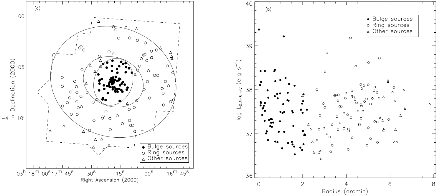
FIG. 3.— (a) Point-source spatial distributions for the 75 bulge sources (filled dots), 71 ring sources (open dots), and 23 other sources (triangles). The dashed boundary lines shows the ACIS-S3 coverage of NGC 1291. (b) Full-band luminosity vs. distance to the nucleus of the galaxy.
