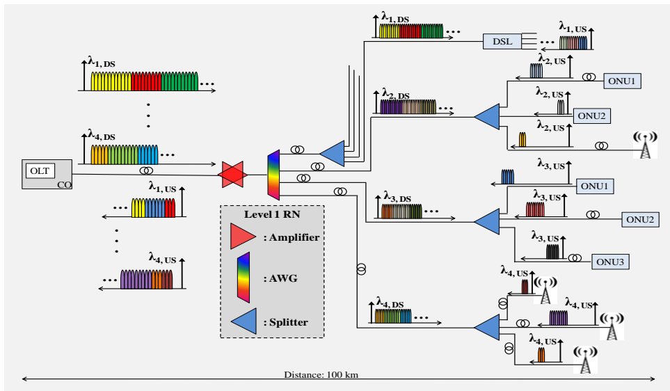
Figure 1. The ACCORDANCE Network.
