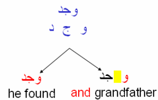
Figure 2: Segmentation Ambiguity
