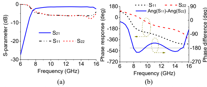
Fig. 4. HFSS-simulated S-parameter responses of (a) magnitude and (b) phase of the proposed unit cell under the normal-impinging TE and TM waves.
