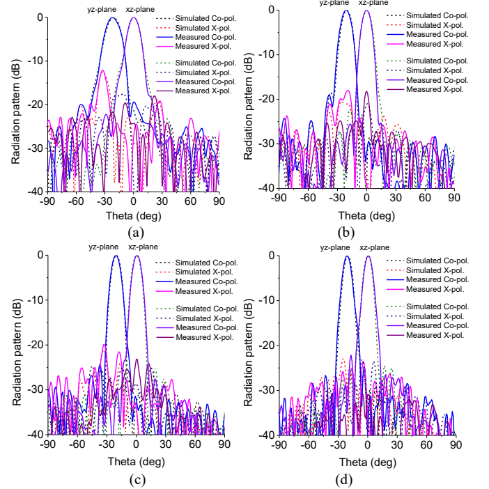
Fig. 12. Normalized radiation patterns of the proposed CP RA antenna in yz-plane and xz-plane (in the beam direction) at (a) 8 GHz, (b) 10 GHz, (c) 12 GHz, and (d) 14 GHz.
