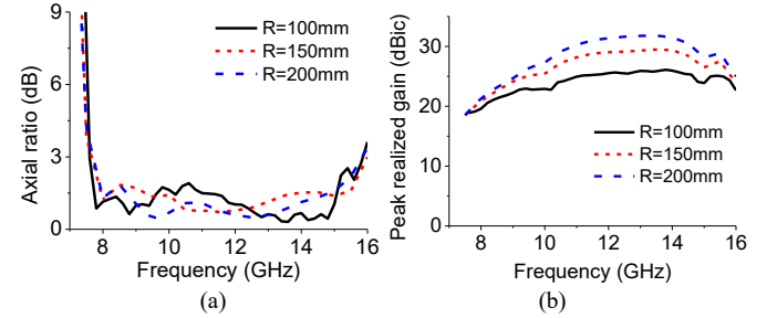
Fig. 9. Performances of (a) AR and (b) peak realized gain of the designed RA antenna with different aperture sizes.
