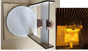
Fig. 10. Photographs of the fabricated CP RA antenna.
