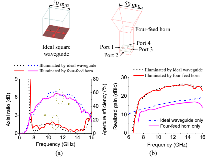
Fig. 8. Performances of (a) AR and AE and (b) peak realized gain of the presented RA antenna when illuminated by different feed antennas.
