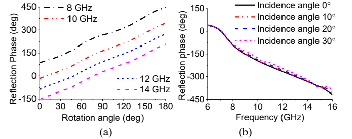
Fig. 6. HFSS-simulated reflection phase of the proposed unit cell with (a) different rotation angles and (b) different incident angles.
