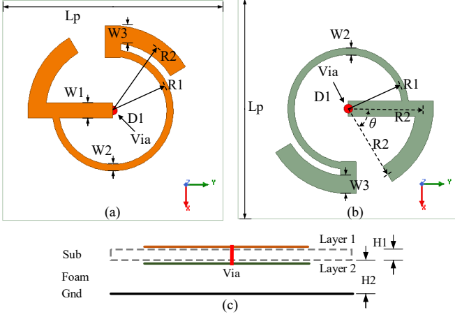
Fig. 1. Configuration of the wideband unit cell for CP radiation. (a) Top Layer. (b) Lower layer. (c) Side view. (Detailed parameters in the design, L_p=10 mm, D1=0.4 mm, W1=0.7 mm, W2=0.3 mm, W3=0.8 mm, R1=2.6 mm, R2=3.5 mm, \theta=59^\circ , H1=0.508 mm, H2=3 mm.)
