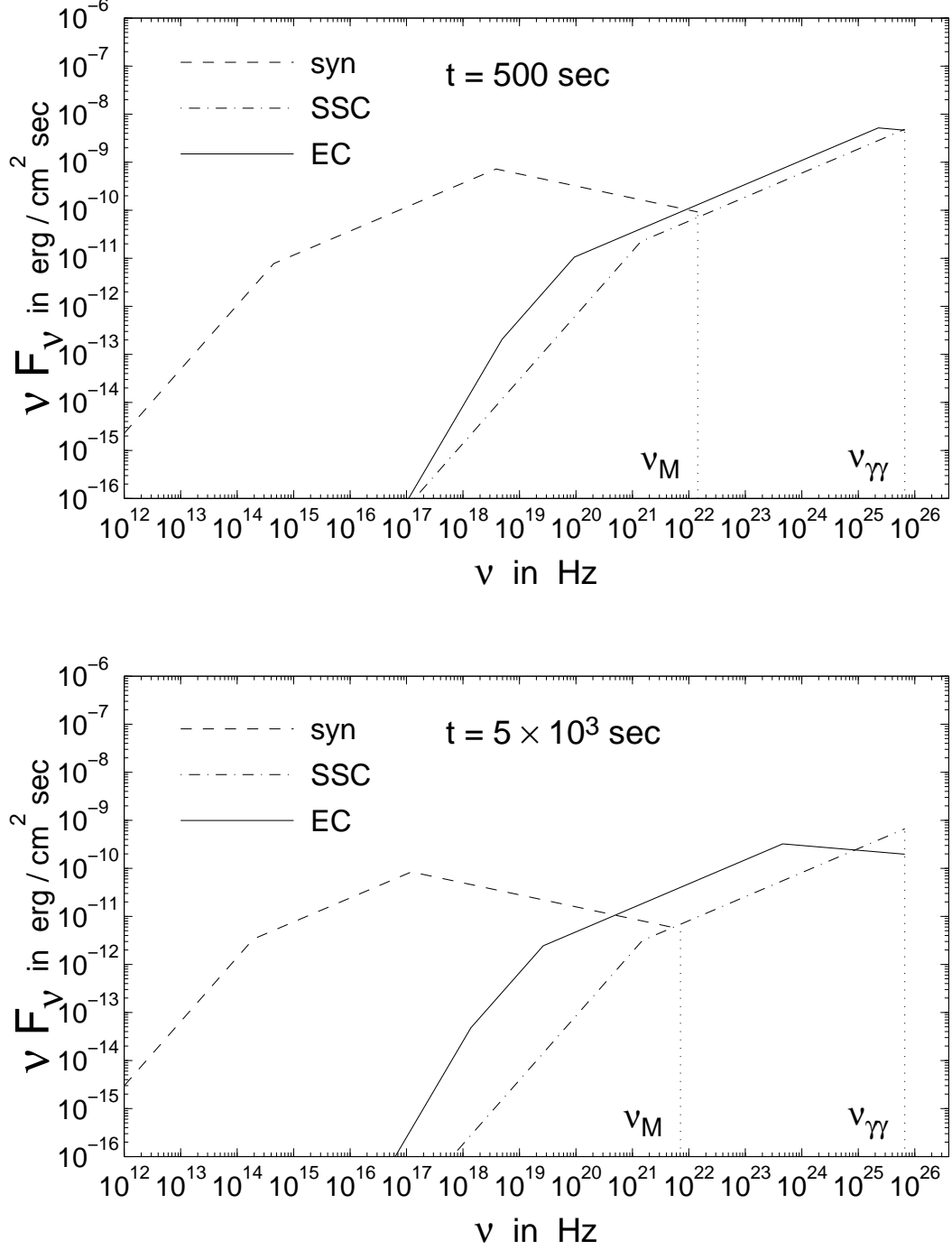
Fig. 2.— The afterglow \nu F_\nu spectrum at t = 500 \text{ s} (upper panel) and 5 \times 10^3 \text{ s} (lower panel) after the GRB, for our fiducial parameters, and for t_{\text{sd}} = 20 \text{ yr} , E_{\text{rot},53} = 0.5 , z = 1 , R_s/R_b = 0.1 . Dotted vertical lines indicate \nu_M where the upper cutoff for the synchrotron emission is located, and \nu_{\gamma\gamma} where the upper cutoff of the SSC and EC (due to pair opacity) is located.
