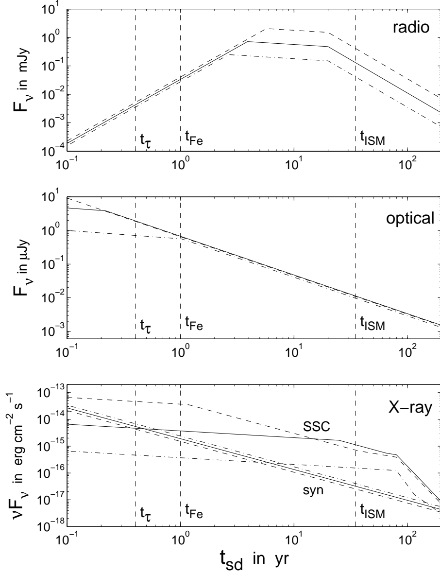
Fig. 1.— The flux density, F_{\nu} , of the plerion emission at the time of the GRB (i.e. a time t_{\text{sd}} after the supernova event), as a function of t_{\text{sd}} . The three panels show the flux density in the radio, optical and X-ray bands ( \nu = 5 \times 10^9 , 5 \times 10^{14} , 10^{18} Hz, respectively). For the radio and optical we show F_{\nu} of the synchrotron emission, and for the X-ray we show \nu F_{\nu} for both the synchrotron and SSC components. The dashed, solid and dot-dashed lines represent \log_{10}(\gamma_w) = 4 , 4.5 and 5, respectively. Dashed lines are shown at t_{\tau} (below which the Thomson optical depth is larger than unity), t_{\text{Fe}} (below which iron line features can appear in the X-ray spectrum of the afterglow) and t_{\text{ISM}} (for which the effective density of the PWB is similar to that of a typical ISM, i.e. 1 \text{ cm}^{-3} ).
