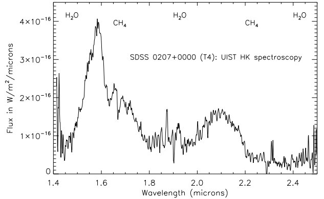
Figure 4. UKIRT/UIST near-infrared spectrum ( HK grism; 1.4–2.5 microns) of a bright T4.0 dwarf (SDSS0207) selected photometrically from the UKIDSS LAS DR1 and confirmed spectroscopically. The discovery 1.0–2.5 microns spectrum is presented in Geballe et al. (2002).
