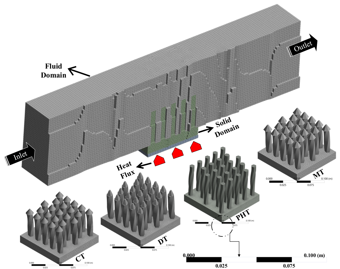
Fig. 5. 3D Mesh visualisation of fluid and solid domains for the pin-fins.
