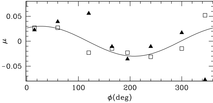
Fig. 9. Distribution of the difference between the peak of magnitudes (squares) and colours (triangles) of C stars within 8 sectors and their average of a unique ellipse with a semi-major axis of 0.7^\circ versus PA (see text for details). The best fit sinusoid has a half amplitude of 0.03 \pm 0.01 mag and corresponds to \phi = 28^\circ \pm 6^\circ . This angle is measured on the plane of the galaxy where 0^\circ corresponds to the NE point of the major axis and increasing to the East. Errors on each point are at most 0.02 mag and have been omitted for clarity.
