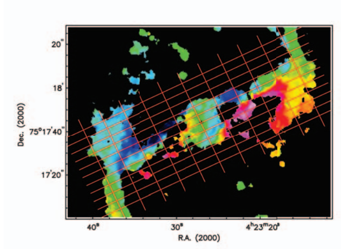
Fig. 7. Lines tracing the cross-sections perpendicular and parallel to the bar of NGC 1530 represented in Figs. 6a to 6d over a portion of the residual velocity map.
