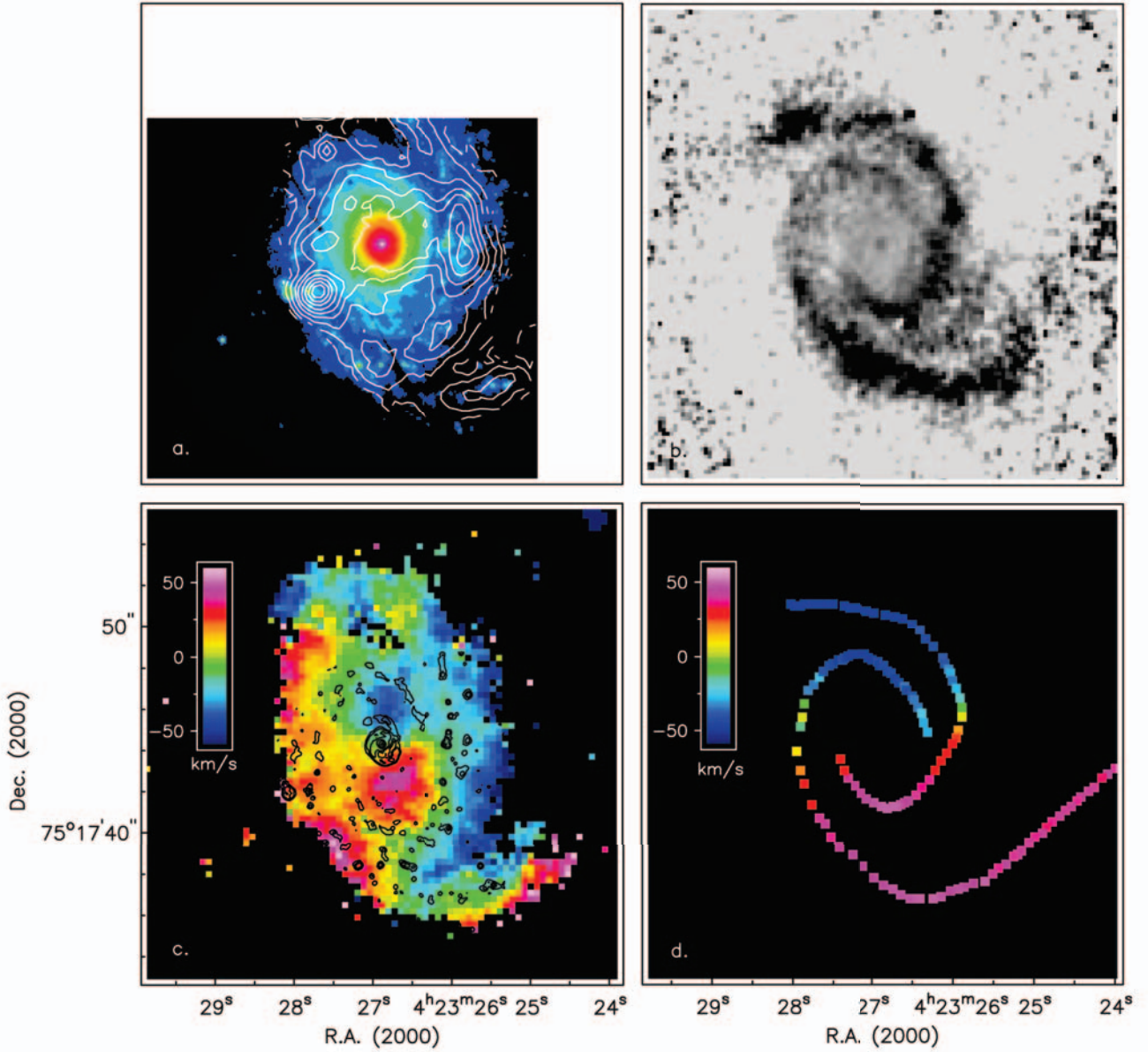
Fig. 14. a) HST –NICMOS H band image of the central part of NGC 1530 with H\alpha isointensity contours overlaid at 1'' resolution. b) Grey-scale representations of the J – K colour index image. Redder colours are indicated by the darker shades. Image taken from Fig. 2 of Pérez-Ramírez et al. (2000). c) Residual velocity map of 1'' resolution of the central part of NGC 1530. This map was obtained after subtracting the model velocity field obtained from the modified rotation curve in the center from the velocity map (see text details). Superposed are isointensity contours of the unsharp mask from the HST –NICMOS image shown in Fig. 15. d) Projected velocity field in the line of sight assuming a gas flow of constant amplitude ( 60 \text{ km s}^{-1} ) along the observed dust lanes (Fig. 14b) in the inner part of NGC 1530. All images, a) to d) , show the same area of the centre of NGC 1530.
