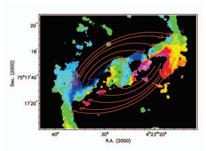
Fig. 8. Schematic representation of the gas orbits along the bar on the residual velocity map, illustrating the dependence of the gas trajectories on orbit semi-minor axis.
