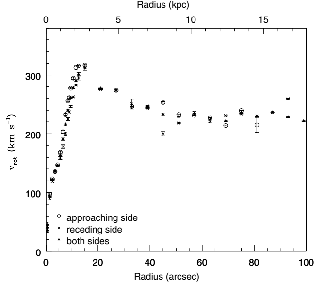
Fig. 2. \text{H}\alpha rotation curve of the disc of NGC 1530, for the receding and the approaching sides of the galaxy separately. The agreement between the two sides shows the symmetry of the velocity field and the reliability of the rotation centre.
