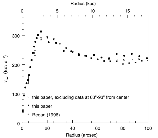
Fig. 5. H\alpha rotation curve of the disc of NGC 1530. This rotation curve has been obtained by subtracting the effect of the streaming motions in the spiral arms of the galaxy from the mean rotation curve shown in Fig. 3 (see text for further details).
