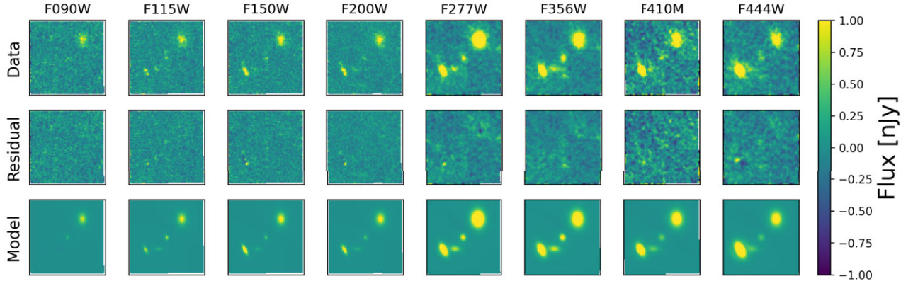
Figure A1. NIRCam imaging across eight filters (top row) in the neighbourhood of JADES-GS-z8-1-LA at z \simeq 8.72 (source on the bottom left, resolved into two components in the SW filters). The FORCEPHO model of the scene (Appendix A) is shown in the bottom row, with residuals shown in the middle row. Note these cutouts are in detector coordinates, with different orientation from Fig. 6.
